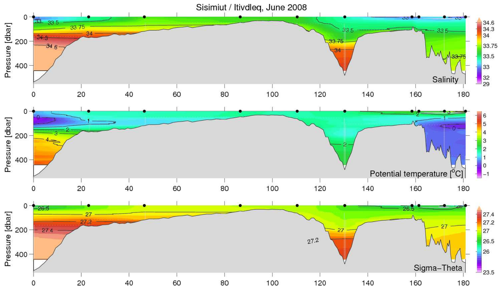
Figure 41. Vertical distribution of temperature, salinity and density at the Itivdleq fjord, June 13–14, 2008. Sisimiut section left (identical to Figure 30).
