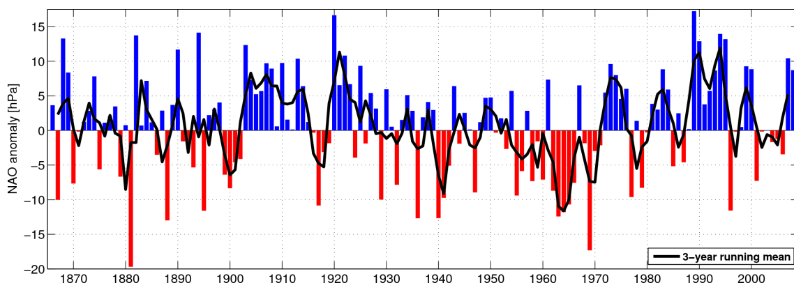
Figure 8. Time series of winter (December–March) index of the NAO from 1865/1866–2007/2008. The heavy solid line represents the NAO index smoothed with a 3-year running mean filter to remove fluctuations with periods less than 3 years. In the figure the winter 1865/1866 is labelled 1866 etc.. The mean and standard deviation is 0.9 \pm 7.3 hPa. Data updated, as described in Buch et al. (2004), from http://ww.cru.uea.ac.uk/cru/data/nao.htm .
