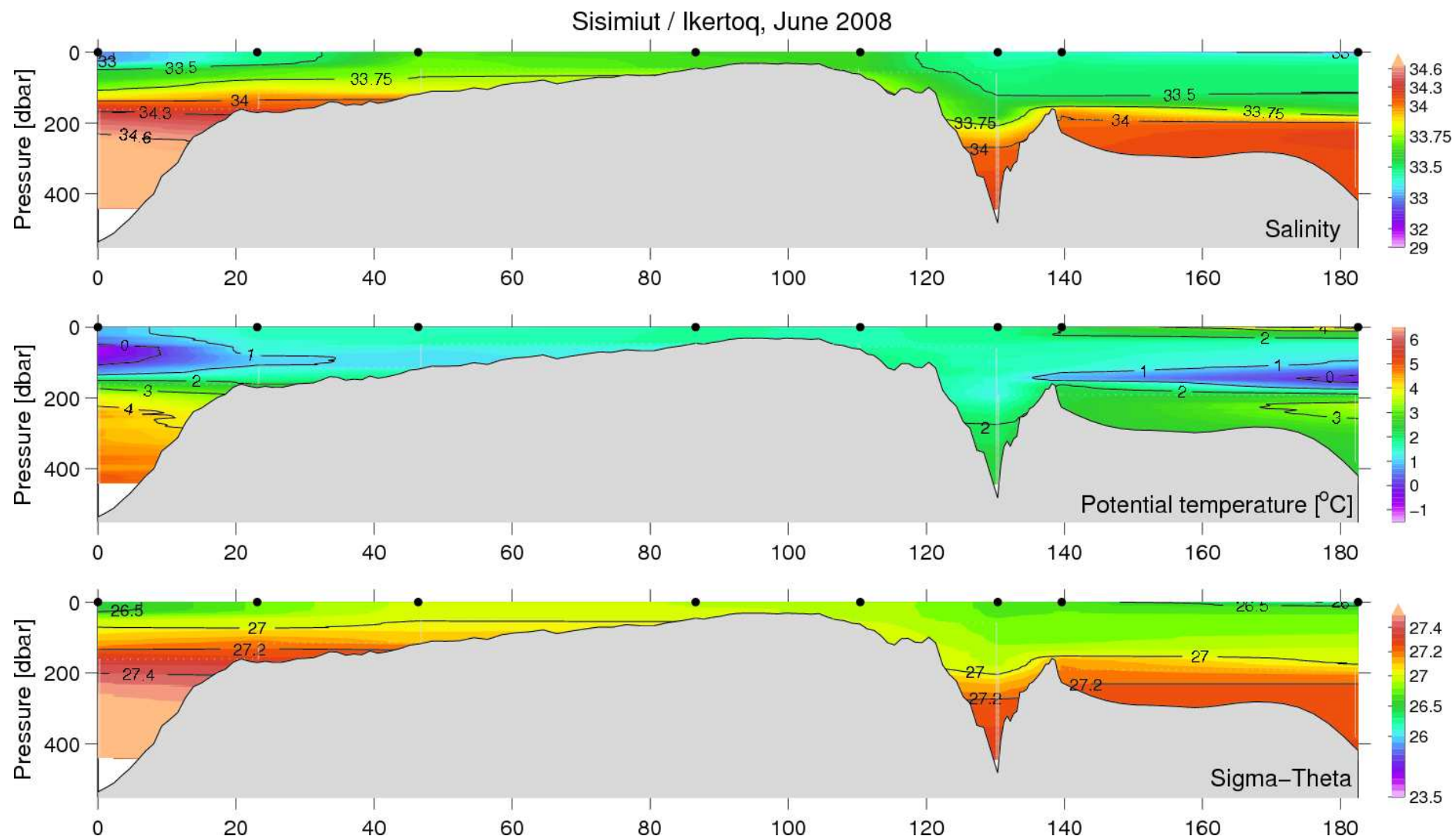
Figure 39. Vertical distribution of temperature, salinity and density at the Ikertoq fjord, June 13–14, 2008. Sisimiut section left (identical to Figure 30).
