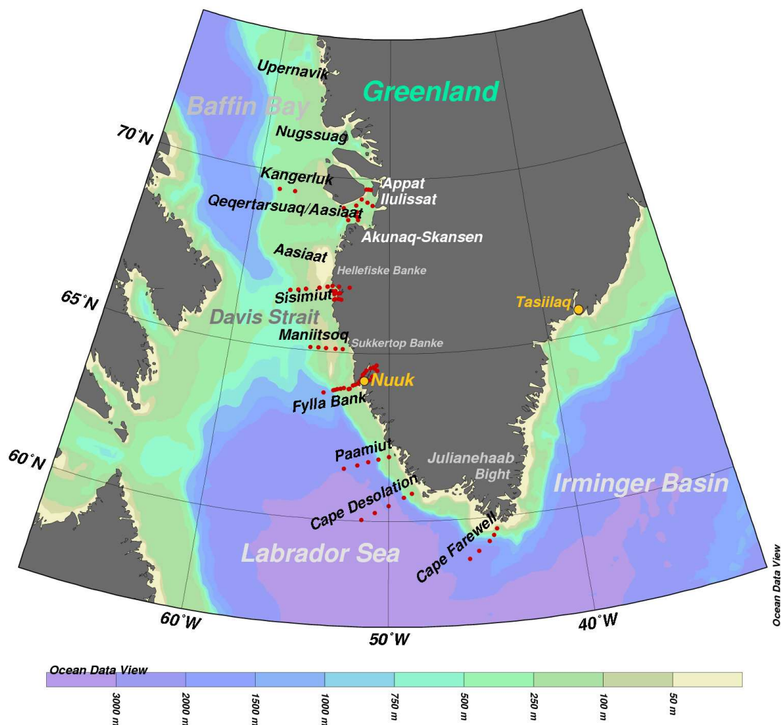
Figure 1. Position of the oceanographic sections off West Greenland where measurements were performed in 2008 except ECOGREEN stations done onboard R/V DANA (Figure 6). The fjord sections at Sisimiut and Godthaabsfjorden are shown in Figure 4 and Figure 5. Contours shown for water depths in colours. Map produced using Ocean Data View (Schlitzer, 2007).
