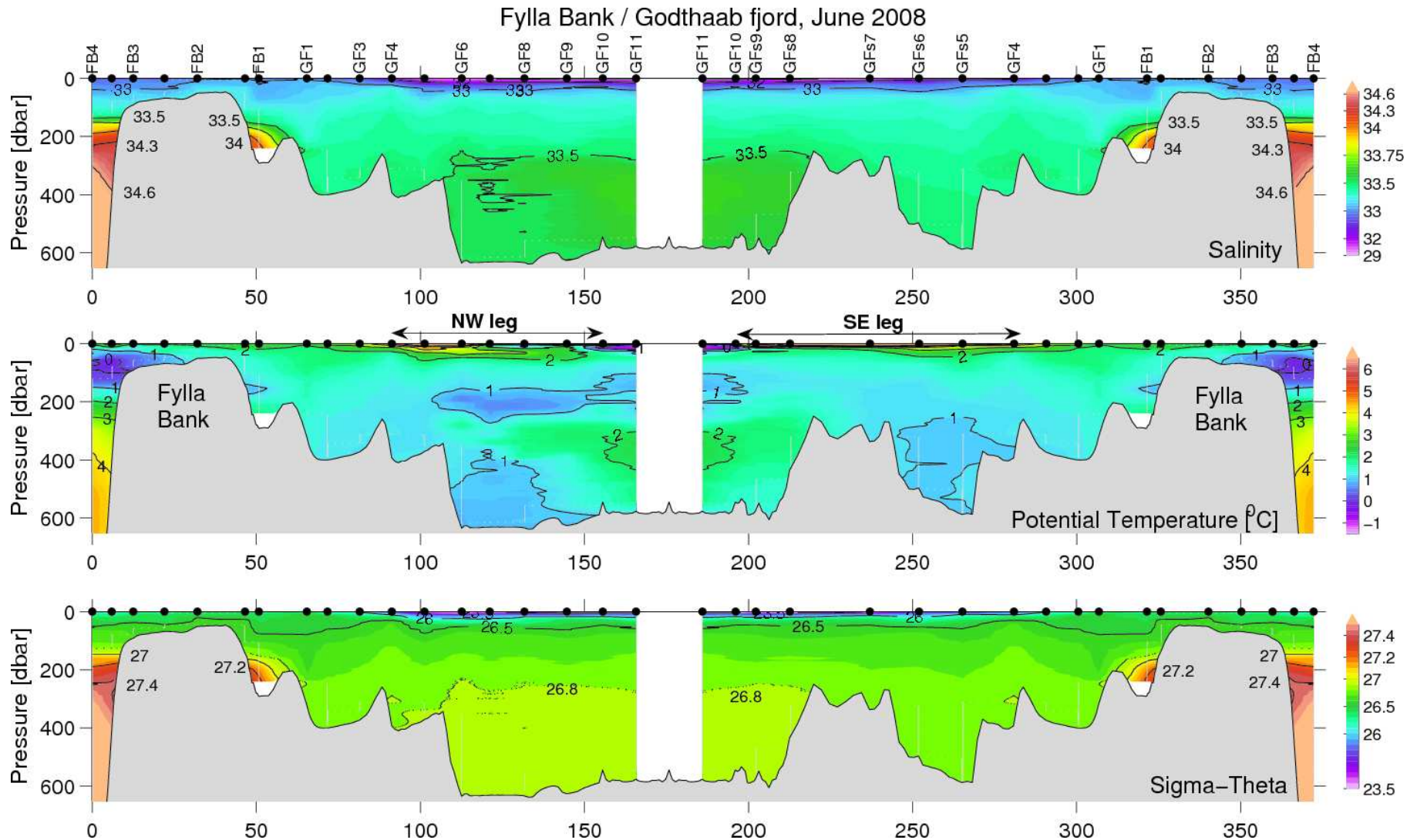
Figure 37. Vertical distribution of temperature, salinity and density at the Fylla Bank / Godthaab fjord section, June 17–18, 2008. From left to middle is shown Fylla Bank and northwest leg (main leg) of Godthaab fjord. From middle to right is shown southeast leg of Godthaab fjord and Fylla Bank. Location of stations shown in Figure 5. The Fylla Bank section is found left and right in the figure (identical to Figure 28).
