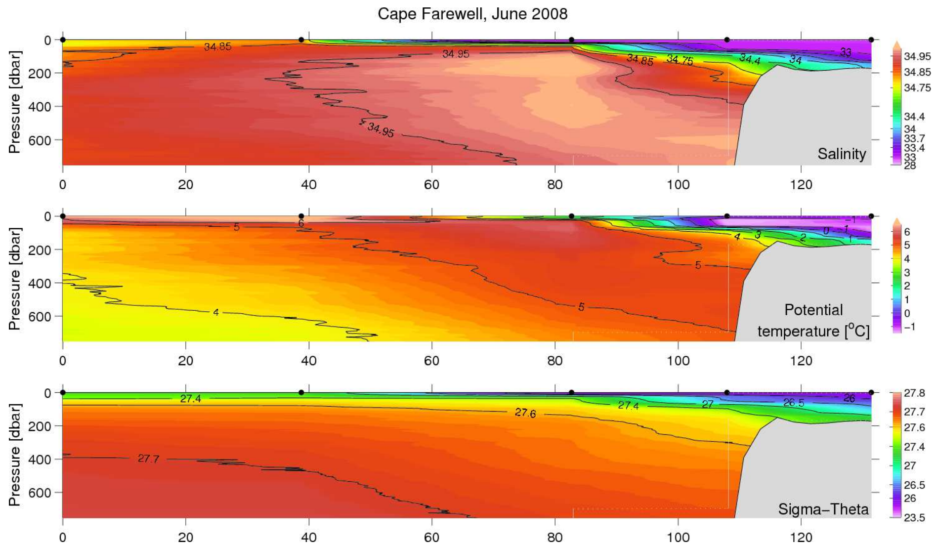
Figure 25. Vertical distribution of temperature, salinity and density at the Cape Farewell section, June 22–23, 2008.
