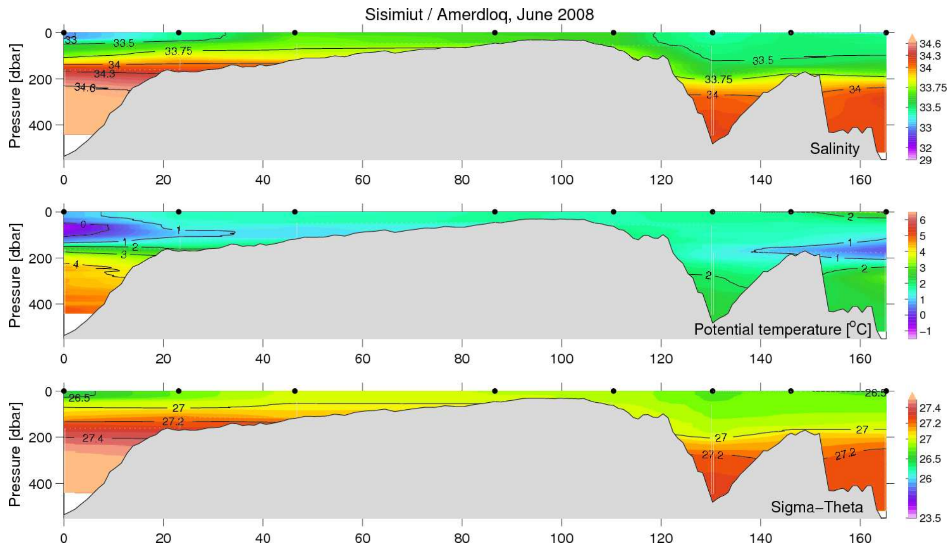
Figure 38. Vertical distribution of temperature, salinity and density at the Amerdloq fjord, June 13–14, 2008. Sisimiut section left (identical to Figure 30).
