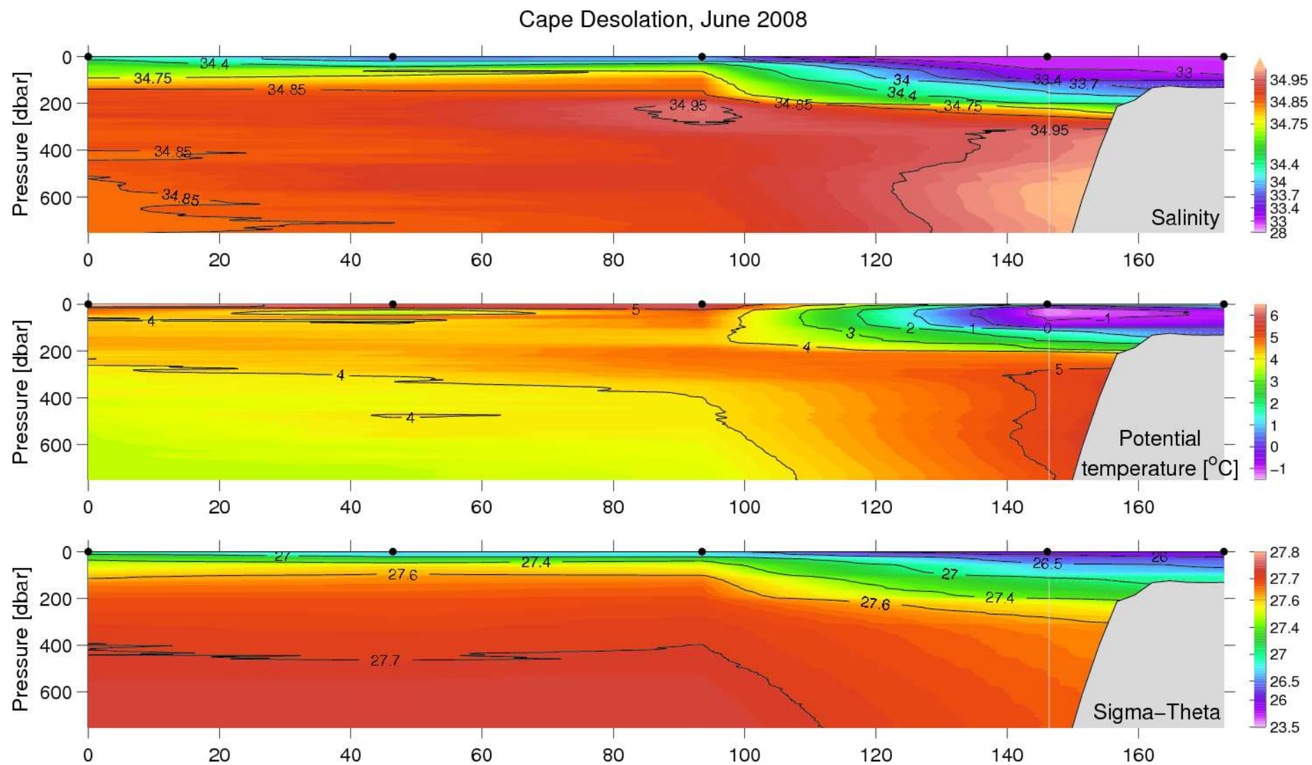
Figure 26. Vertical distribution of temperature, salinity and density at the Cape Desolation section, June 21, 2008.
