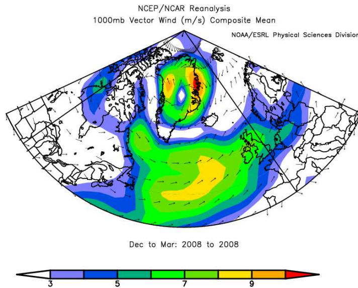
Figure 11. Winter (DJFM) wind for 2007/2008 in the North Atlantic region. NCEP/NCAR re-analysis (from http://www.cdc.noaa.gov ).
