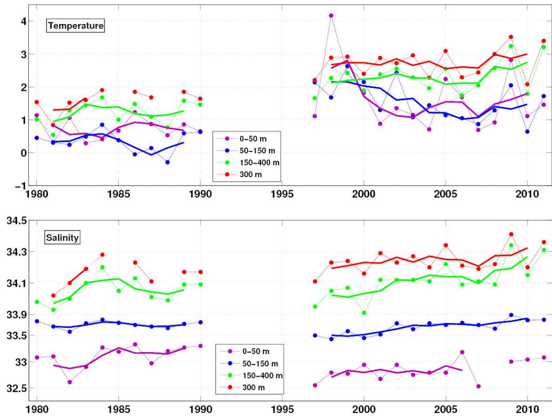
Figure 22. Timeseries of mean temperature (top) and mean salinity (bottom) for the period 1980–2011 in four different depth intervals west of “Jakobshavn-Skansen” (Ilulissat-Skansen) st.3 in the Disko Bay close to Jakobshavn Isbræ. The thick curves are the 3 year running mean values. Note the change in scales at 33.9 for salinity. Statistics is shown in Table 4.
