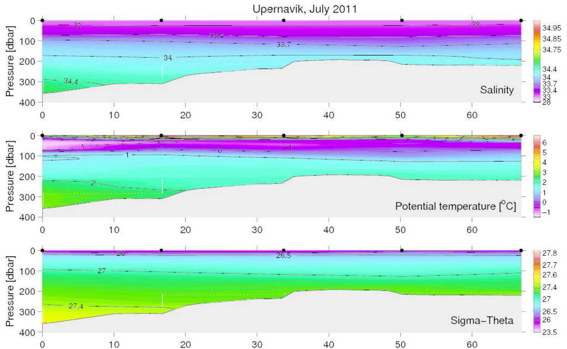
Figure 38. Vertical distribution of temperature, salinity and density at the Upernavik section, July 05, 2011.
