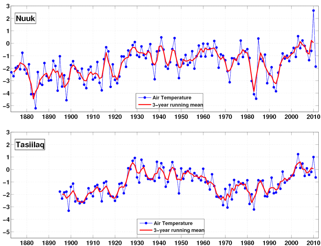
Figure 14. Annual mean air temperature observed at Nuuk and Tasiilaq for the period 1873–2011. The mean and standard deviation is -1.64 \pm 1.25 °C for Nuuk and -1.11 \pm 1.00 °C for Tasiilaq. Values for 2011 are respectively -1.72 °C and -0.64 °C. Nuuk temperature was taken from the Nuuk airport synop station 04254 due to a failure on the instrument (Nuuk synop 04250) for more than 65% of the following months (yyyymm): 200505, 200710, 200712, 200811, 201101.
