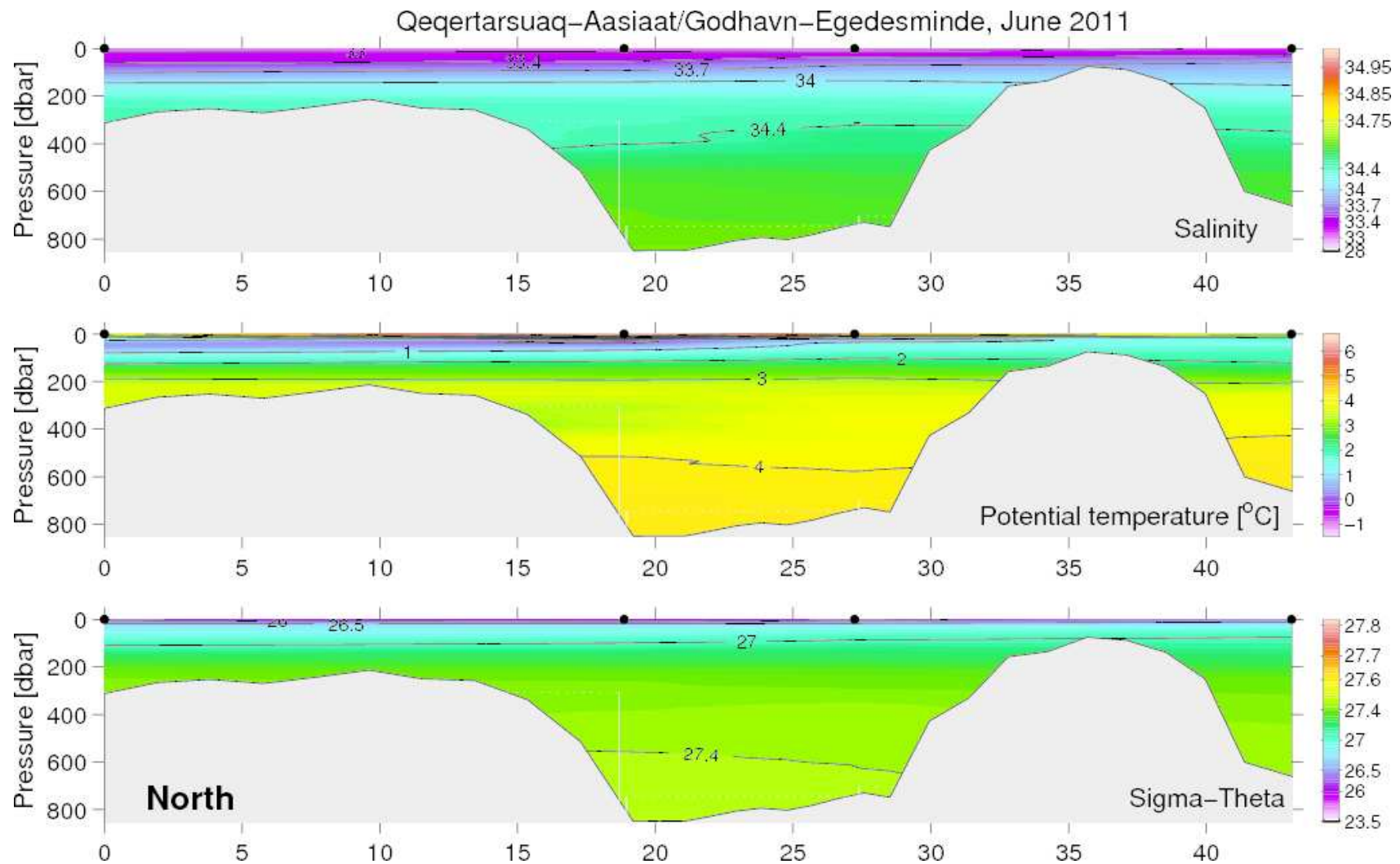
Figure 39. Vertical distribution of temperature, salinity and density at the Aasiaat–Qeqertarsuaq (Egedesminde–Godhavn) section, June 21–22, 2011. Note: The cross section is directed from section 1–4 (see Figure 1). The deep channel (19–28 km) is westward along the deep channel southeast of “Hunde øerne”.
