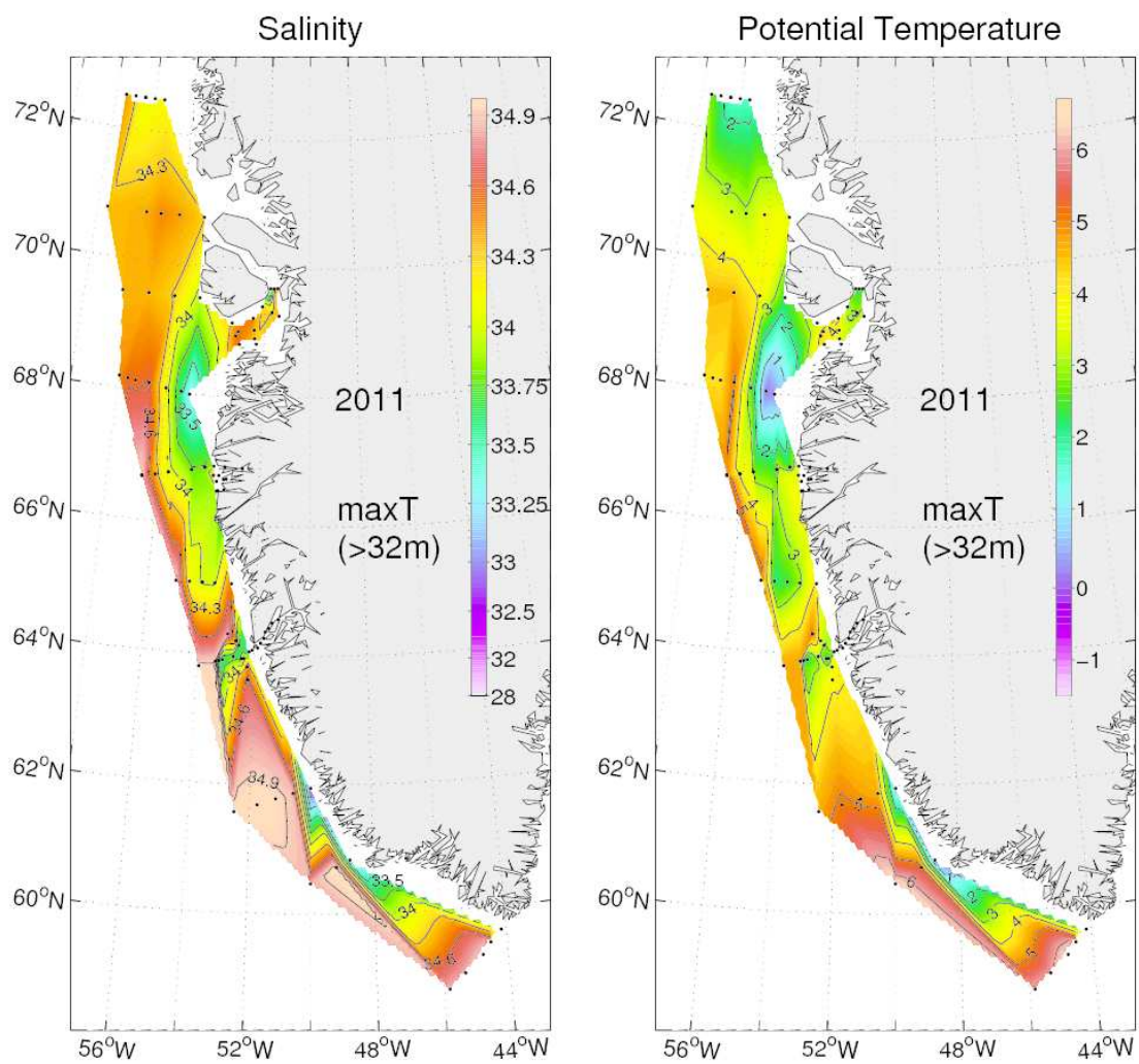
Figure 24. Salinity (left) and temperature (right) observed in 2011 (June 15 – July 13) at the depth of maximum temperature disregarding the upper 32 meters.
