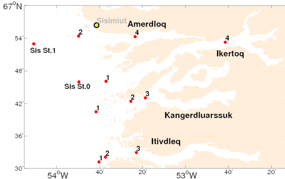
Figure 4. Position of the oceanographic stations around Sisimiut where measurements were performed in 2011. See Figure 1 for position of all sections measured in 2011.
