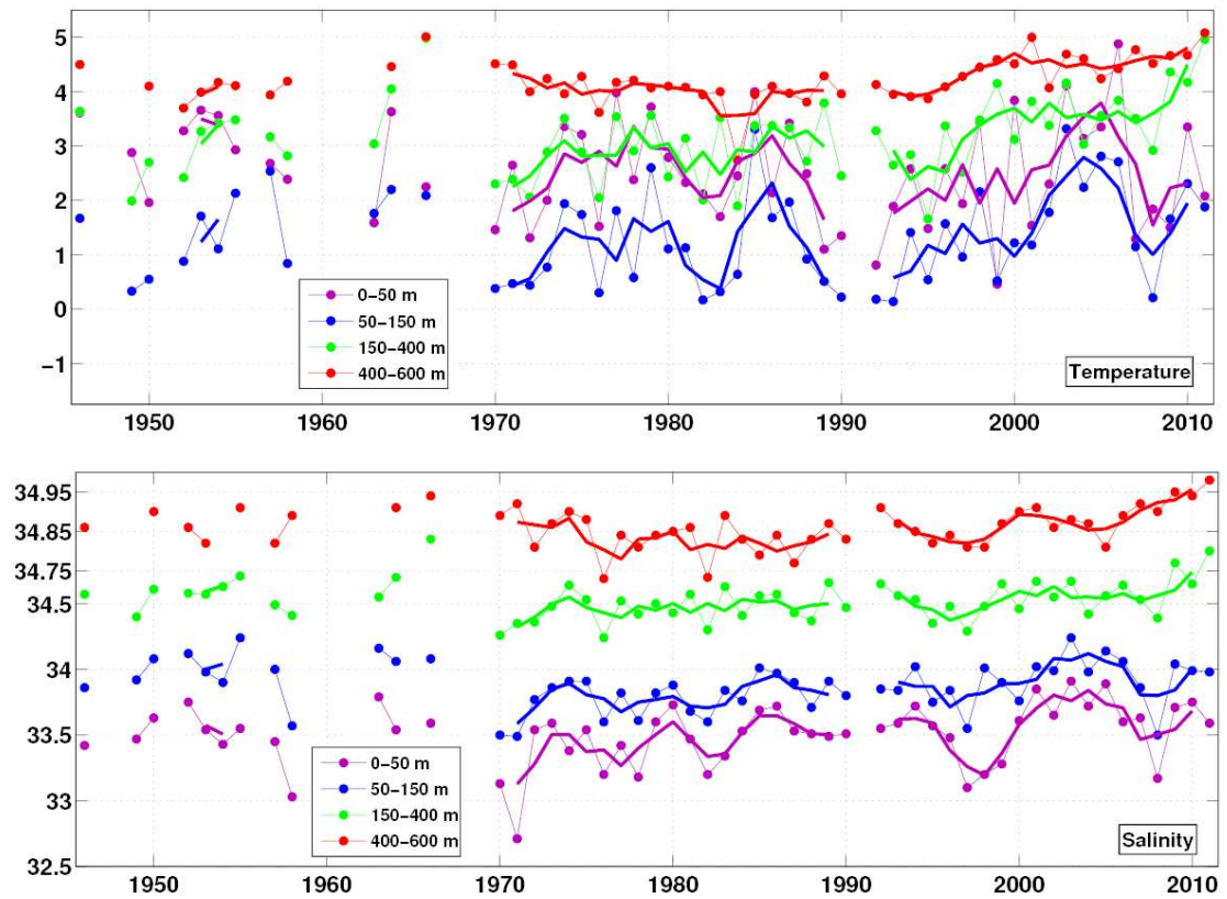
Figure 20. Timeseries of mean temperature (top) and mean salinity (bottom) for the period 1946–2011 in four different depth intervals west of “Sukkertop Banke” (Maniitsoq, st.5) over the continental slope. The thick curves are the 3 year running mean values. Note the change in scales at 34.75 for salinity. Statistics is shown in Table 3.
