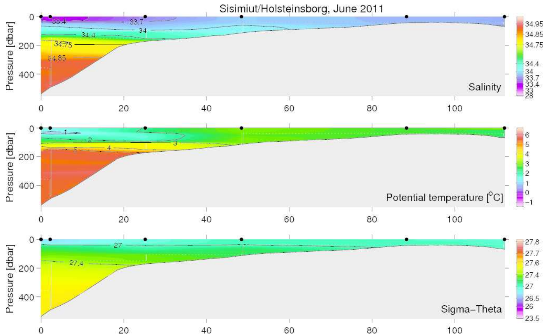
Figure 34. Vertical distribution of temperature, salinity and density at the Sisimiut (Holsteinsborg) section, June 15–16, 2011.
