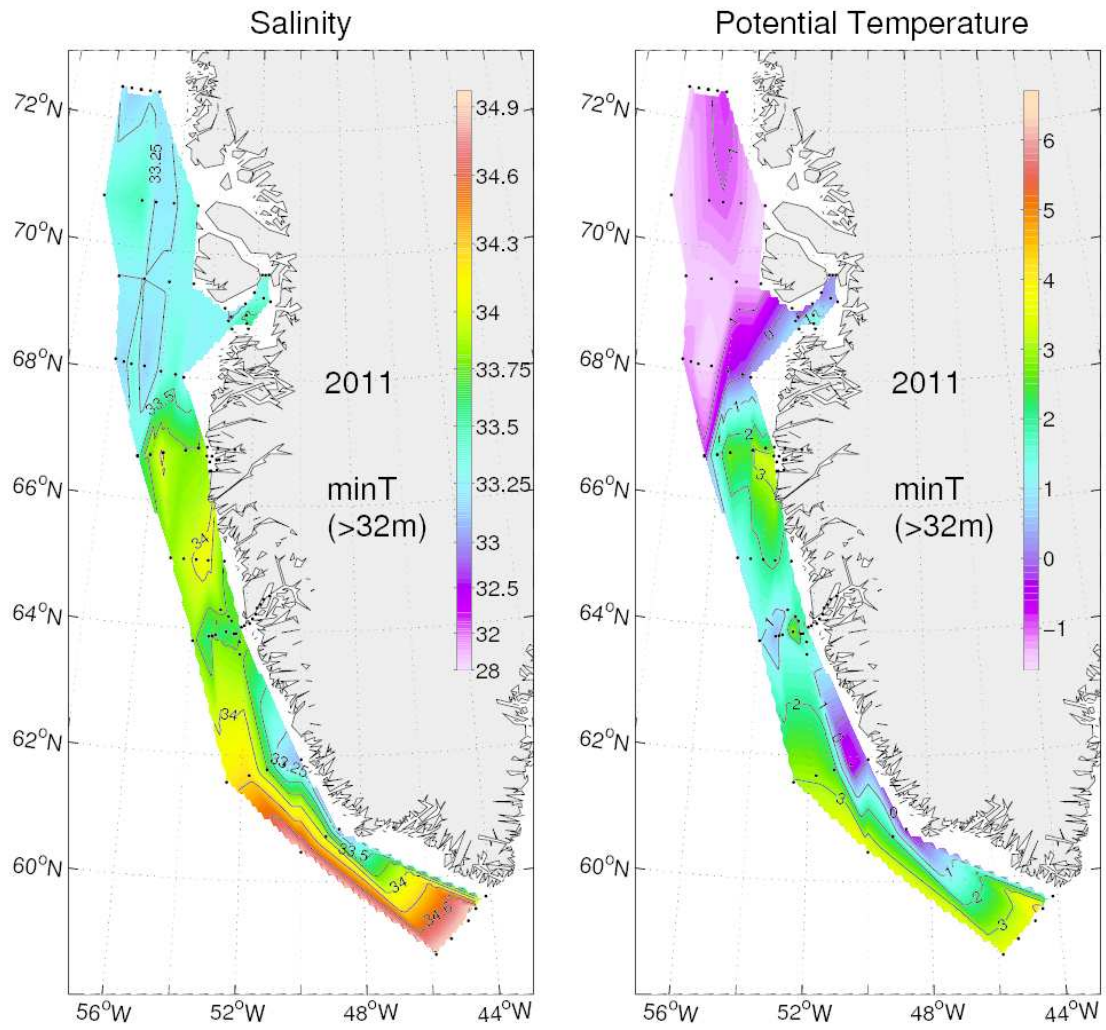
Figure 23. Salinity (left) and temperature (right) observed in 2011 (June 15 – July 13) at the depth of minimum temperature disregarding the upper 32 meters.
