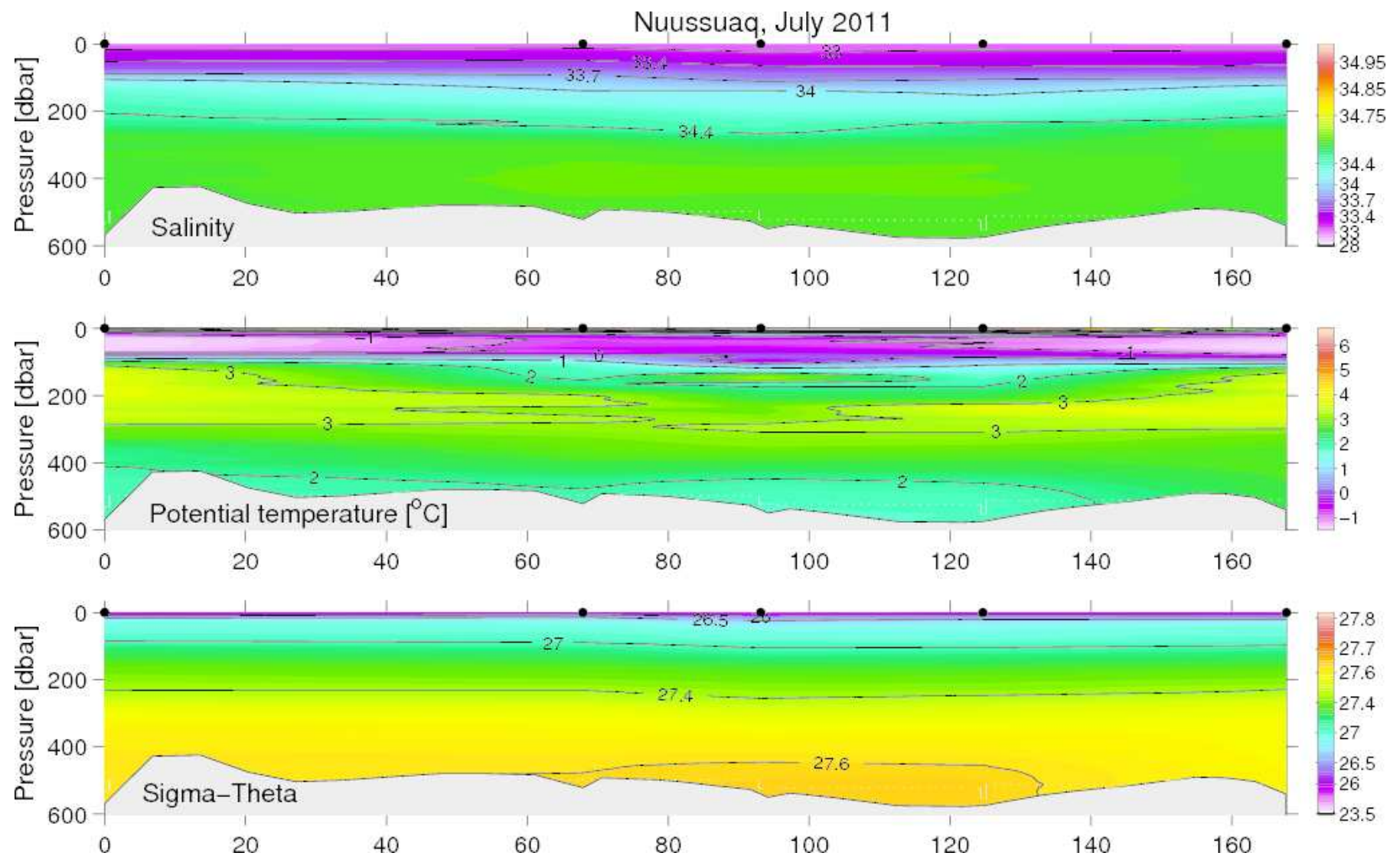
Figure 37. Vertical distribution of temperature, salinity and density at the Nuussuaq section, July 02-07, 2011.
