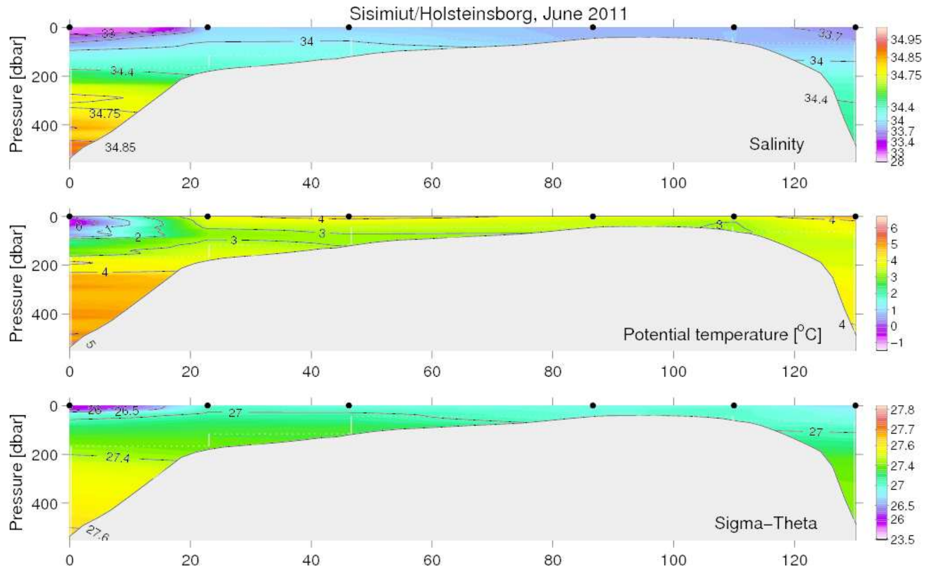
Figure 33. Vertical distribution of temperature, salinity and density at the Sisimiut (Holsteinsborg) section, June 28–29, 2011.
