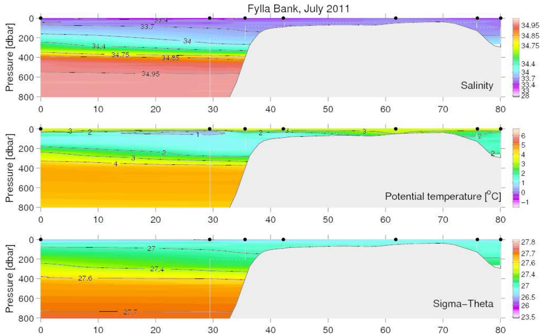
Figure 31. Vertical distribution of temperature, salinity and density at the Fylla Bank section, July 01, 2011. Three intermediate stations were taken too.
