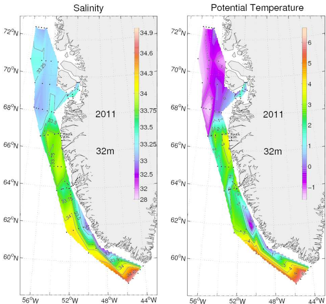
Figure 17. As Figure 16, but for 32 m depth.
