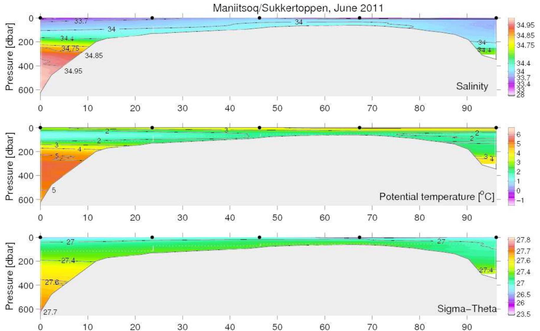
Figure 32. Vertical distribution of temperature, salinity and density at the Maniitsoq (Sukkertoppen) section, June 30, 2011.
