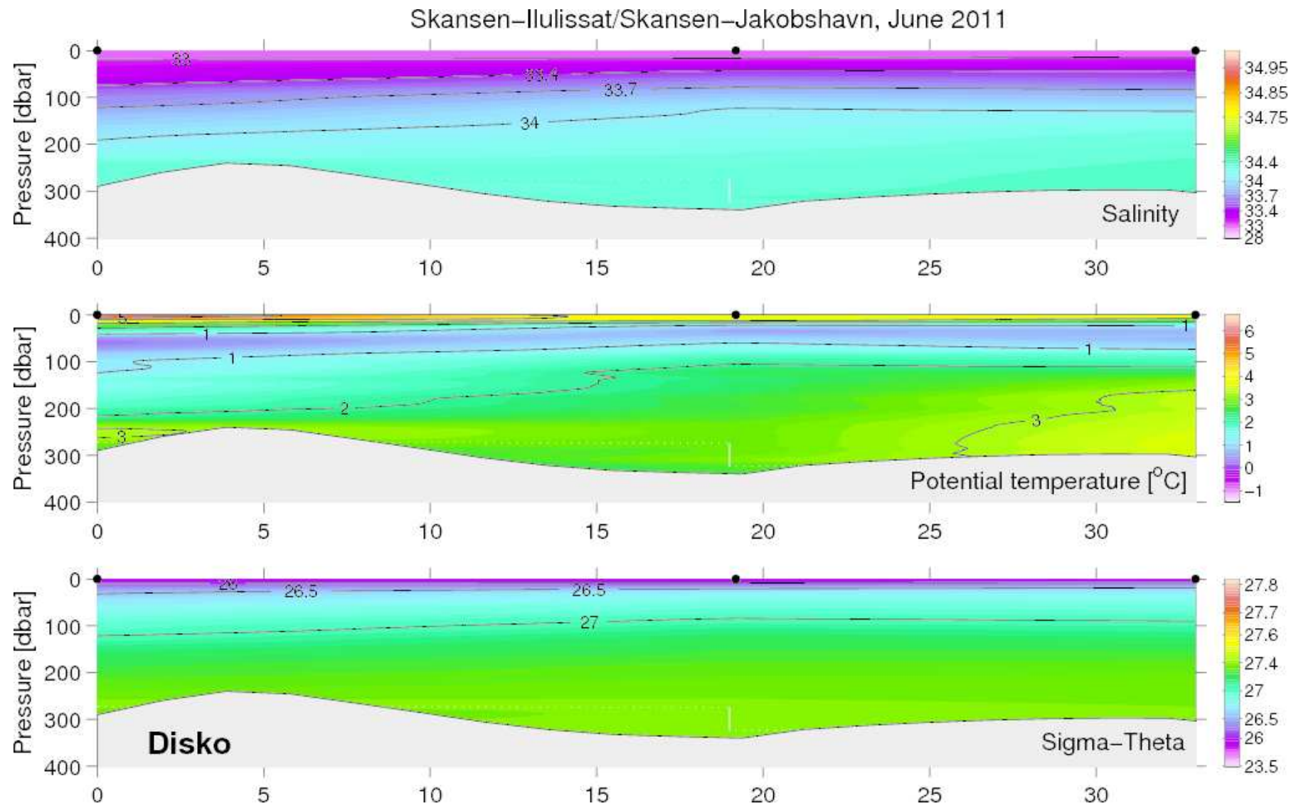
Figure 41. Vertical distribution of temperature, salinity and density at the Skansen–Ilulissat (Skansen–Jakobshavn) section, June 24–25, 2011.
