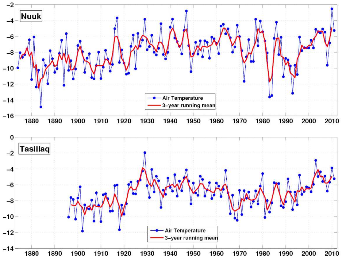
Figure 12. Winter (DJFM) mean air temperature observed at Nuuk and Tasiilaq for the period 1874–2011. The mean and standard deviation for the whole timeseries is -7.9 \pm 2.3 °C for Nuuk and -7.0 \pm 1.8 °C for Tasiilaq. Values for 2011 are respectively -5.26 °C and -5.24 °C. Nuuk temperature was taken from the Nuuk airport synop station 04254 due to a failure on the instrument (Nuuk synop 04250) for more than 65% of the following months (yyyy-mm): 200505, 200710, 200712, 200811, 201101.
