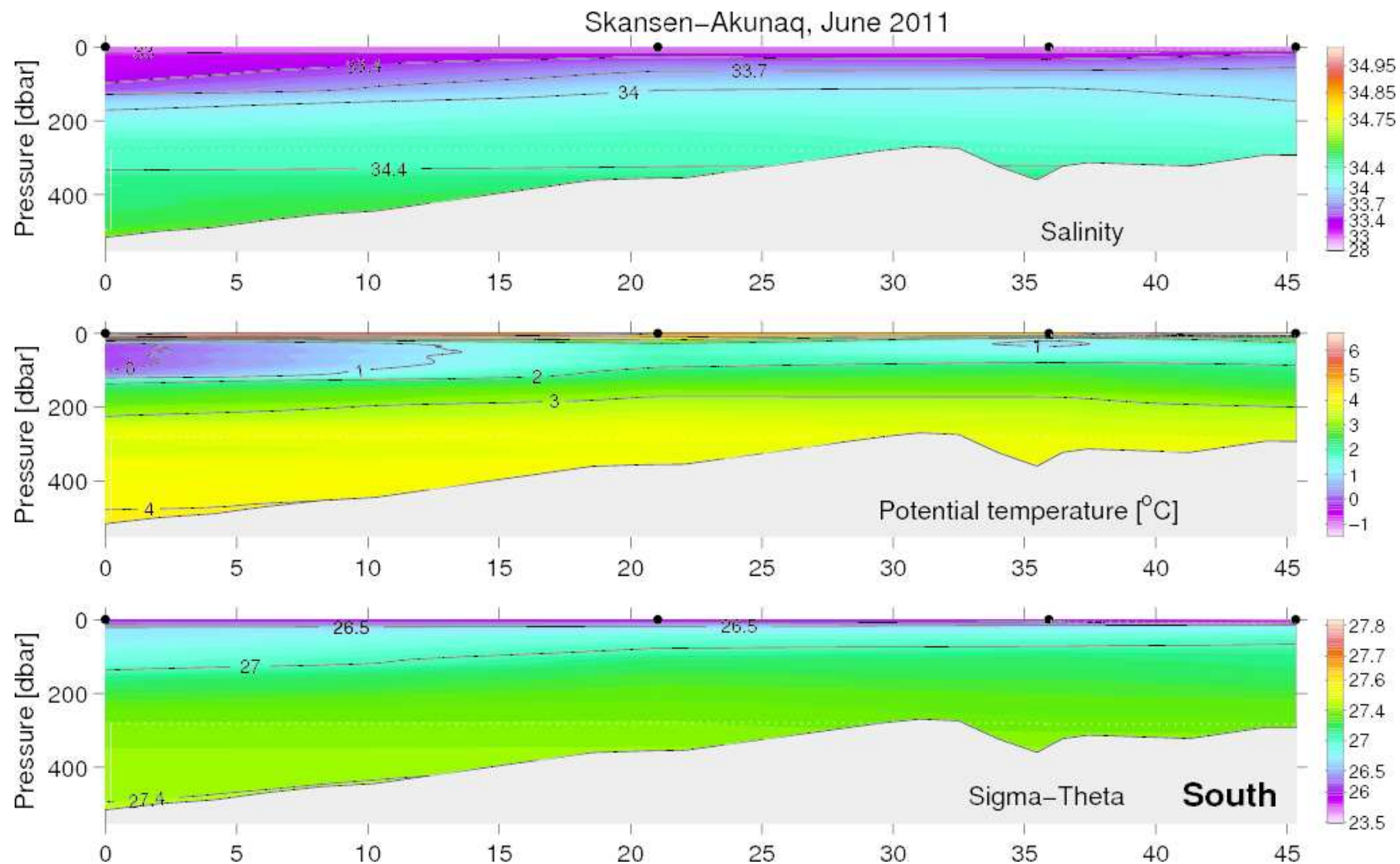
Figure 40. Vertical distribution of temperature, salinity and density at the Skansen–Akunaq section, June 21–24, 2011.
