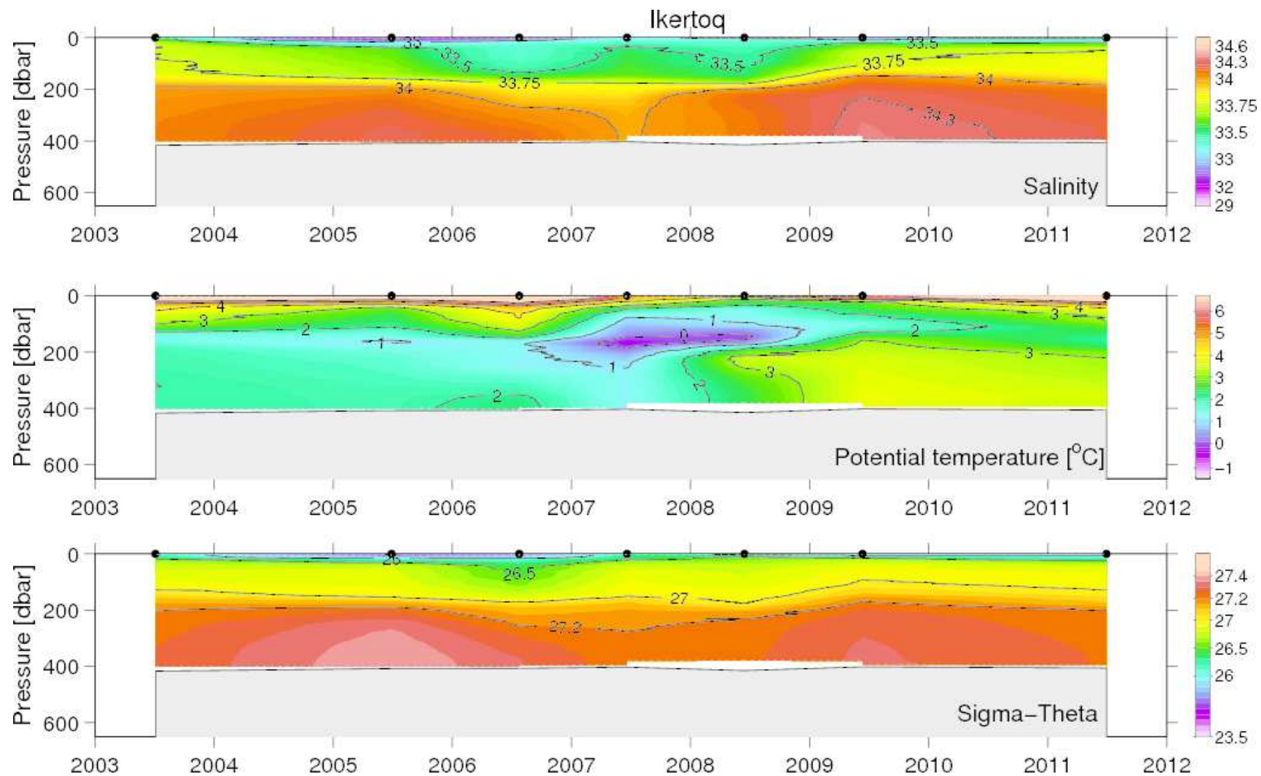
Figure 49. Hovmöller diagram of vertical distribution of temperature, salinity and density at the Ikertoq fjord st.4, late June/July 2003, 2005–2009, 2011.
