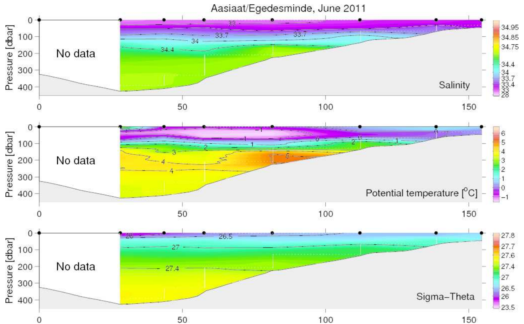
Figure 35. Vertical distribution of temperature, salinity and density at the Aasiaat (Egedesminde) section, June 18–20, 2011.
