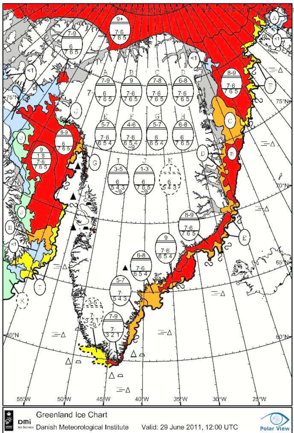
Figure 6. Distribution of sea ice in Greenland Waters valid for 29. June 2011.
