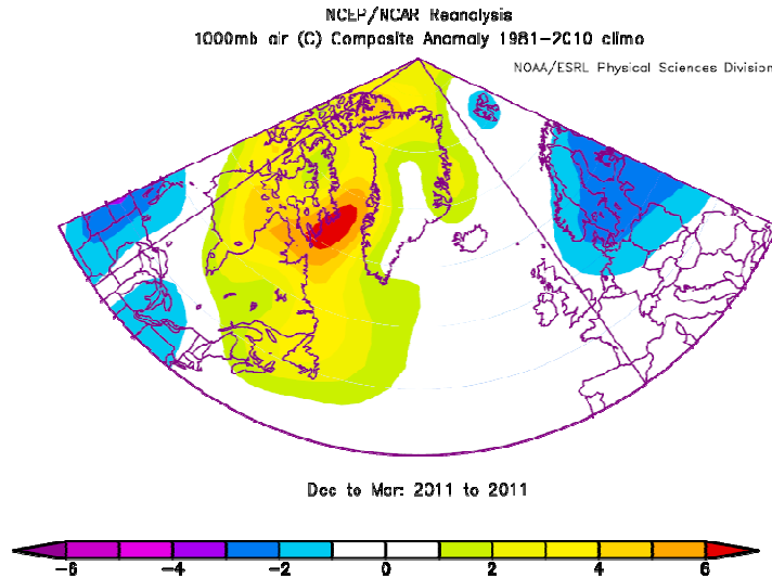
Figure 11. Winter (DJFM) mean air temperature anomaly for 2010/11 in the North Atlantic region. NCEP/NCAR re-analysis (from http://www.esrl.noaa.gov/psd/ ).
