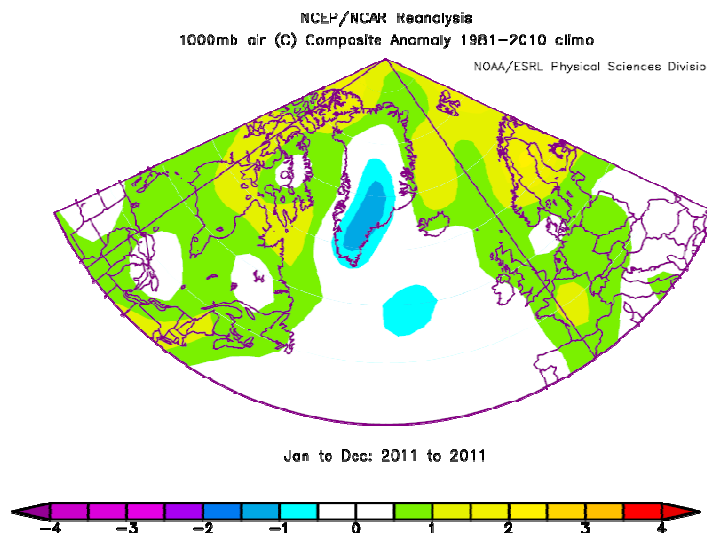
Figure 13. Anomalies of the annual mean air temperature for 2011 in the North Atlantic region. NCEP/NCAR re-analysis (from http://www.esrl.noaa.gov/psd/ ).
