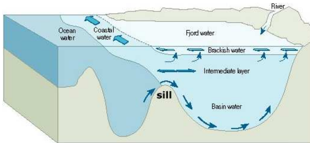
Figure 19. Sketch of the circulation in a fjord (modified from AMAP Assessment Report: Arctic Pollution Issues, Figure 3.20, http://www.amap.no/maps-gra/show.cfm?figureId=58 ).
