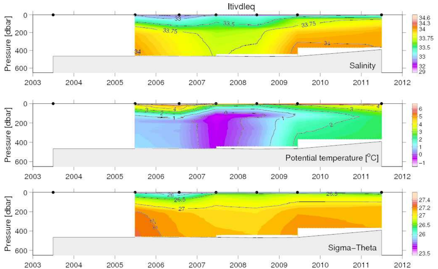
Figure 51. Hovmöller diagram of vertical distribution of temperature, salinity and density at the Itivdleg fjord st.4, late June/July 2005–2009, 2011. Itivdleg St. 3 was used for 2011.
