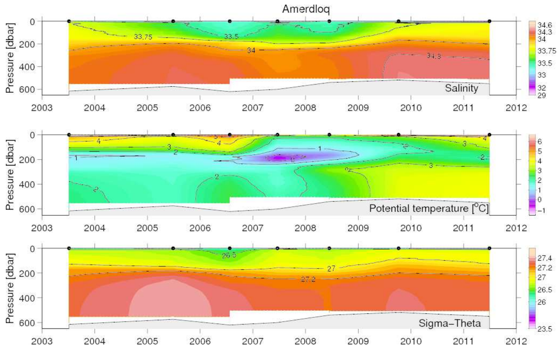
Figure 48. Hovmöller diagram of vertical distribution of temperature, salinity and density at the Amerdloq fjord st.4, late June/July 2003, 2005–2009, 2011.
