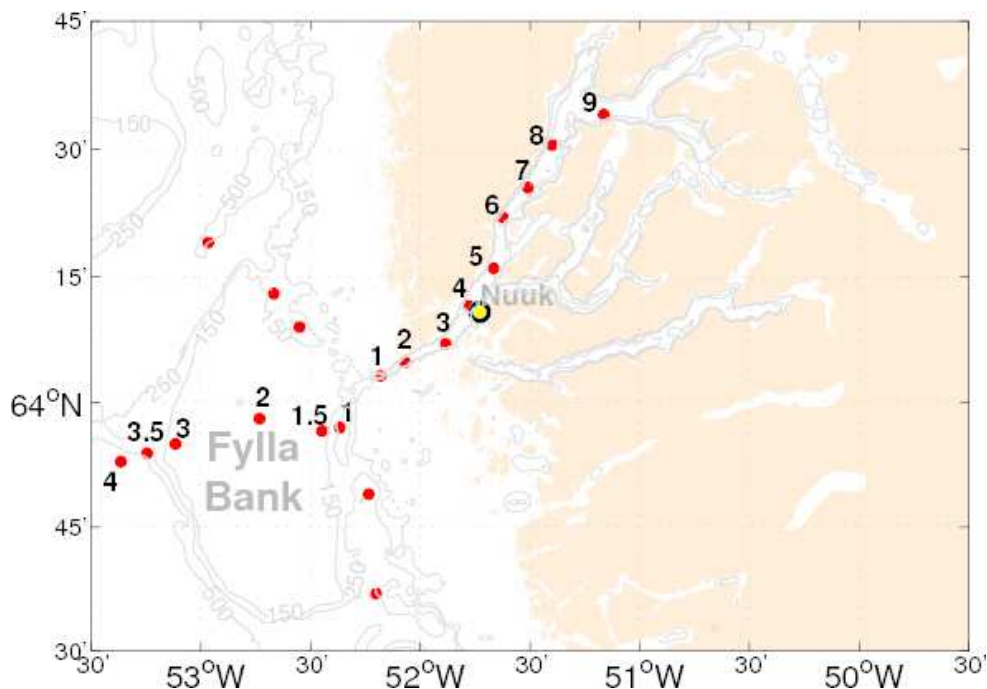
Figure 5. Position of the oceanographic stations in Godthaabfjorden and Fylla Bank. In 2011 measurements were only performed over Fylla Bank and st. 1–9 in the “main arm” of the Godthaabfjorden. The numbers refer to standard station numbers as shown in Figure 43. Moreover some additional stations were taken in the channels east of the Fylla Bank. See Figure 1 for position of all sections measured in 2011.
