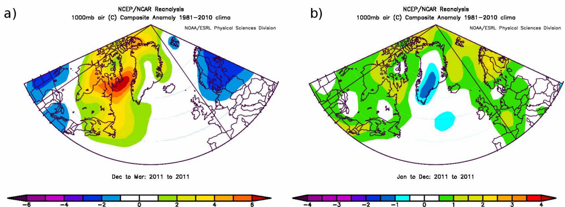
Figure 10. a) Winter (DJFM) mean air temperature anomaly for 2010/11 in the North Atlantic region. b) Annual mean air temperature anomaly for 2011. NCEP/NCAR re-analysis (from http://www.esrl.noaa.gov/psd/ ).
