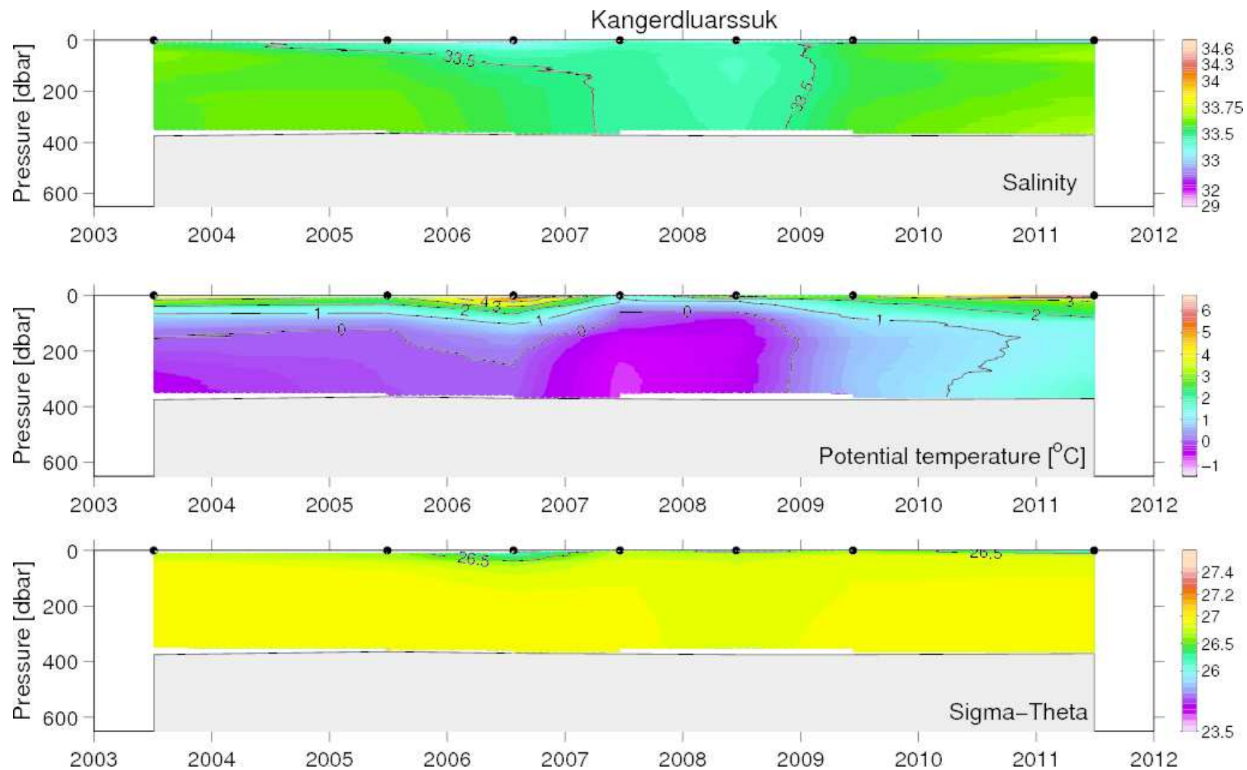
Figure 50. Hovmöller diagram of vertical distribution of temperature, salinity and density at the Kangerdluarssuk fjord st.3, late June/July 2003, 2005–2009, 2011.
