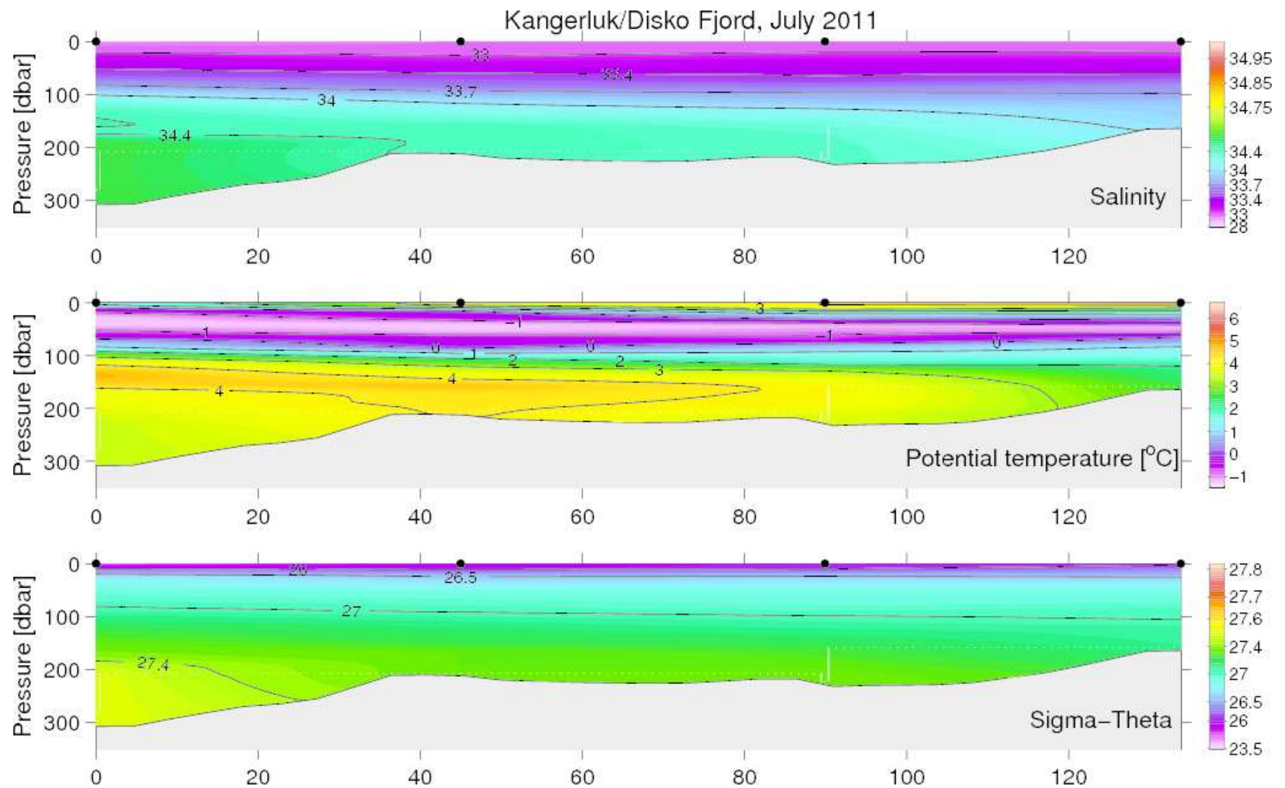
Figure 36. Vertical distribution of temperature, salinity and density at the Kangerluk (Disko Fjord) section, July 01–07, 2011.
