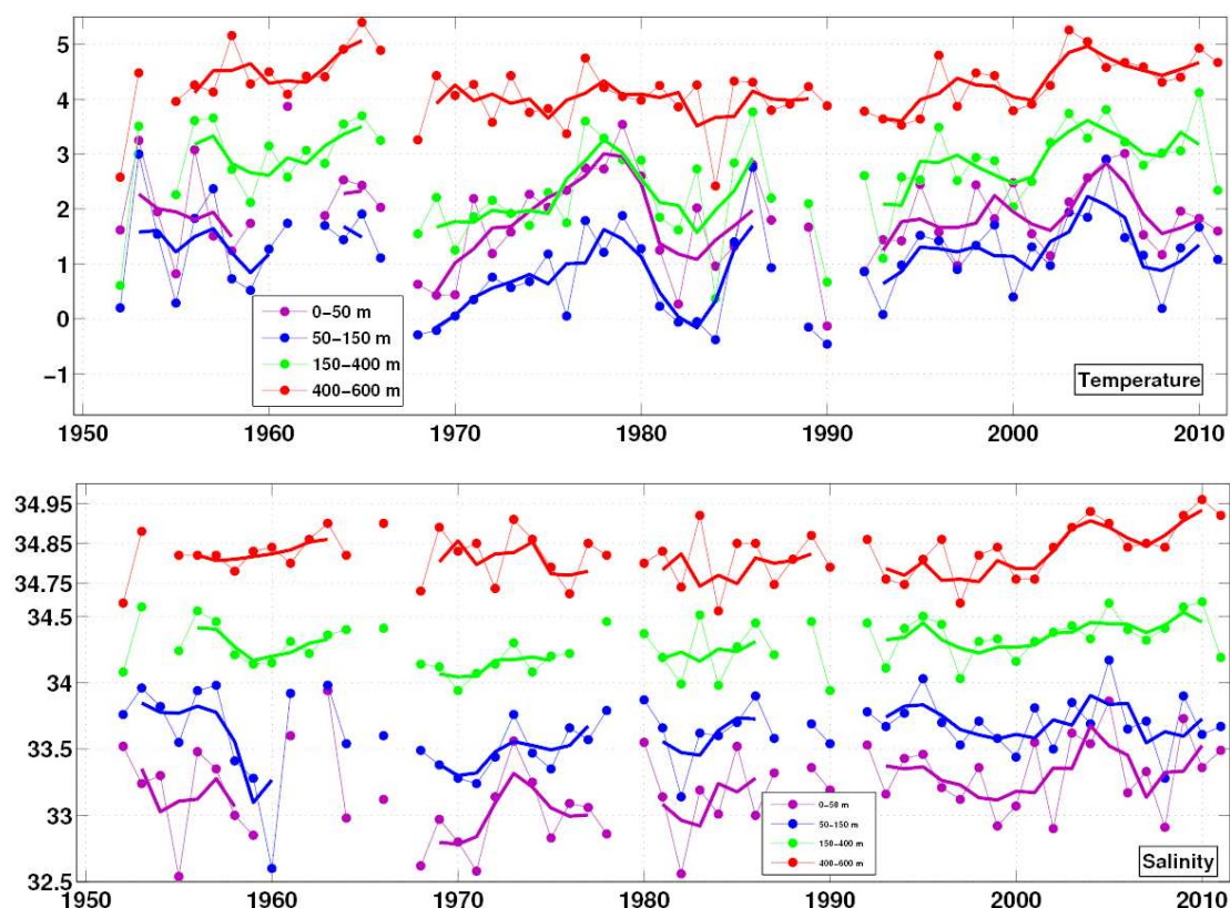
Figure 18. Timeseries of mean June-July temperature (top) and salinity (bottom) for the period 1950–2011 averaged in four different depth intervals west of Fylla Bank (st.4) over the continental slope. Thick curves are the 3 year running mean values. Note the change in scales at 34.75 for salinity. Statistics are shown in Table 2.
