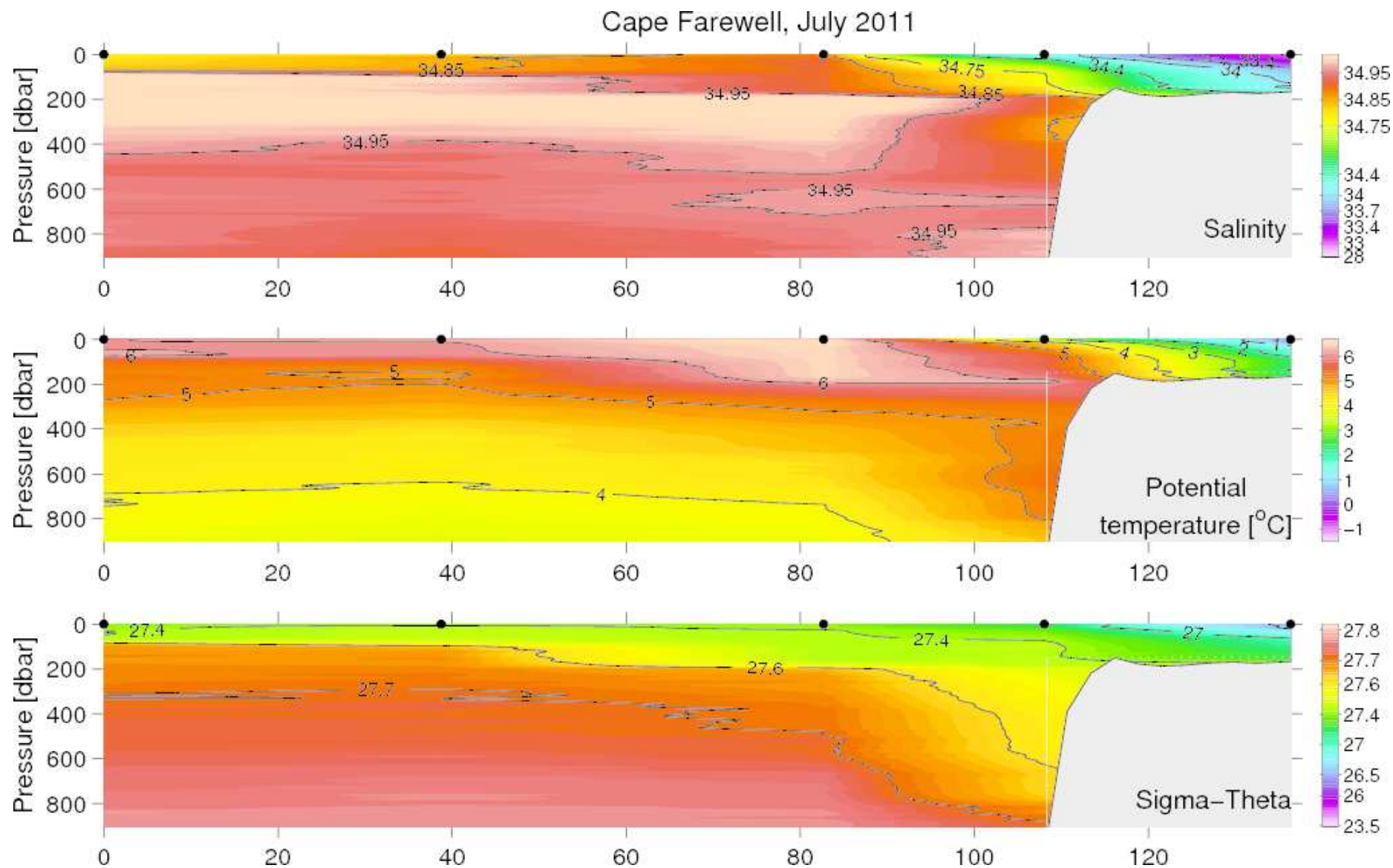
Figure 28. Vertical distribution of temperature, salinity and density at the Cape Farewell section, June 12–13, 2011.
