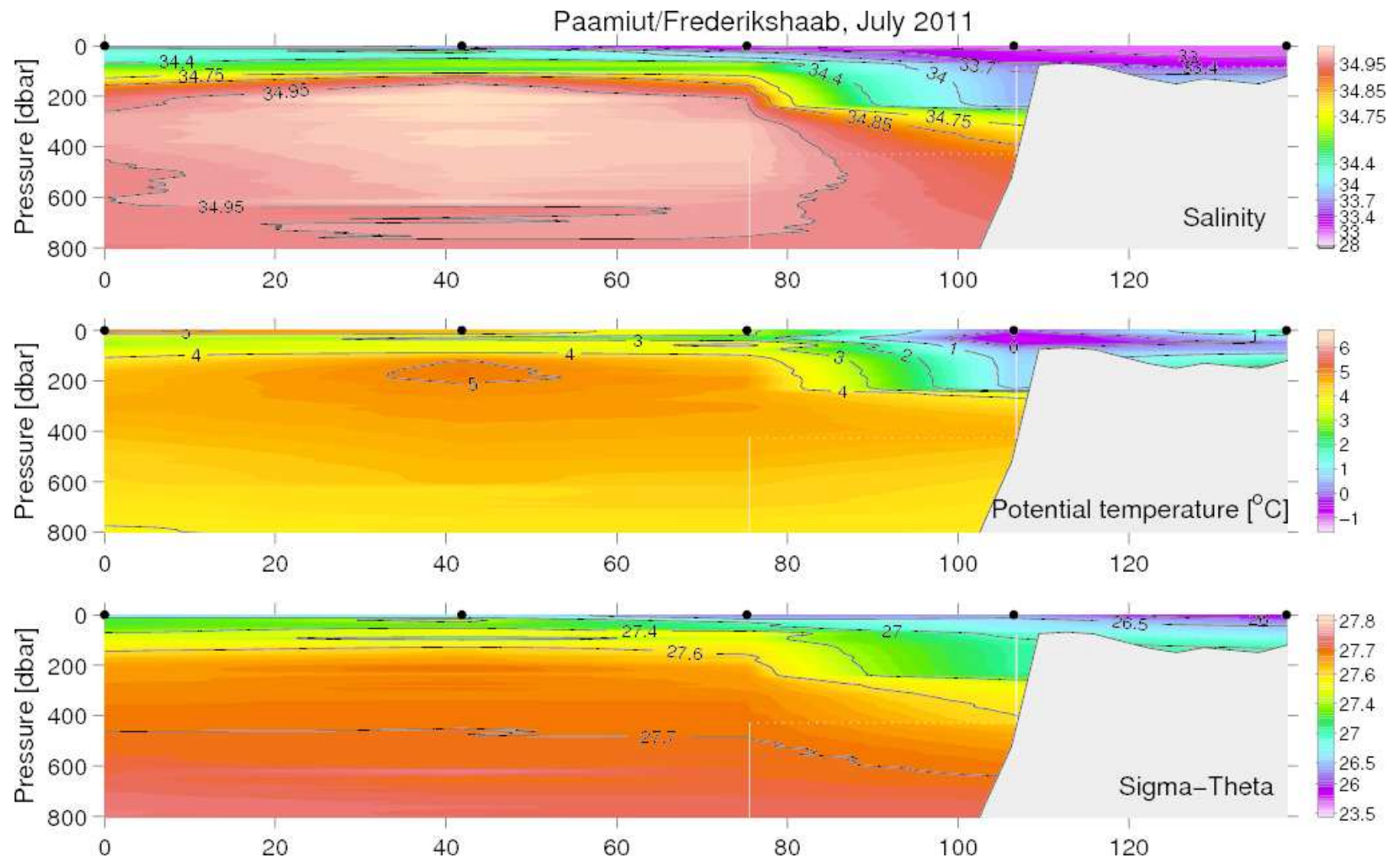
Figure 30. Vertical distribution of temperature, salinity and density at the Paamiut (Frederikshaab) section, July 05, 2011.
