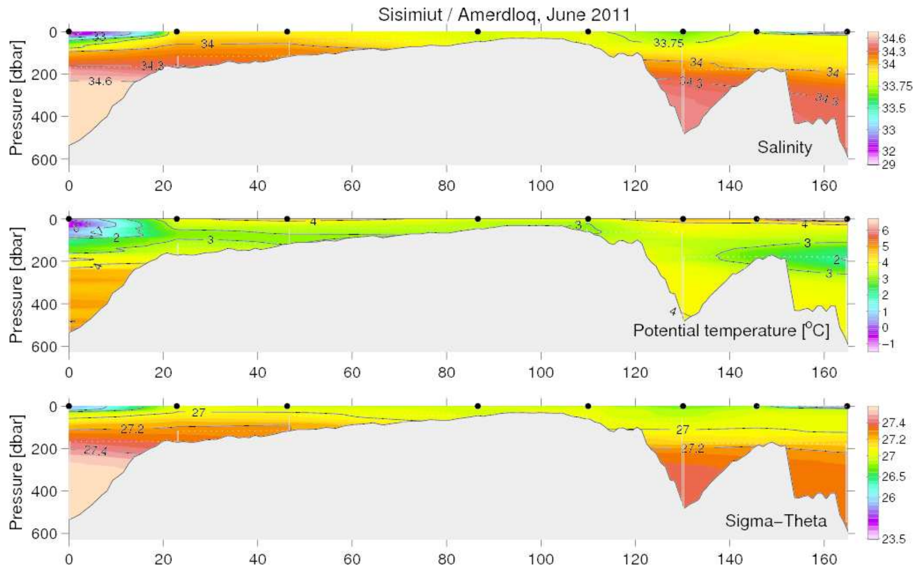
Figure 44. Vertical distribution of temperature, salinity and density at the Amerdloq fjord, June 28–29, 2011. Sisimiut section left.
