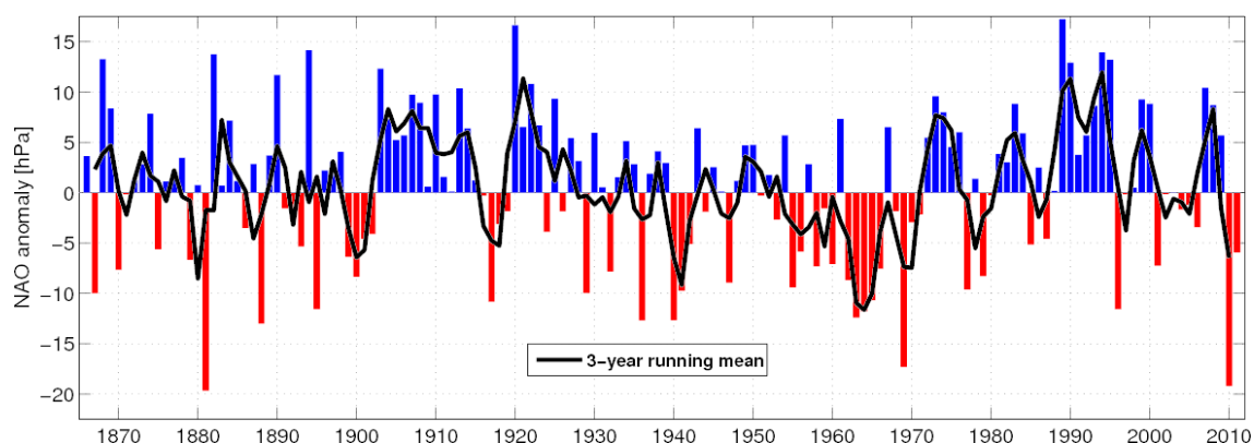
Figure 7. Time series of winter (December–March) index of the NAO from 1865/1866–2010/11. The heavy solid line represents the NAO index smoothed with a 3-year running mean filter to remove fluctuations with periods less than 3 years. In the figure the winter 1865/1866 is labelled 1866 etc.. The mean and standard deviation is 0.71 \pm 7.5 hPa. The 2010/11 value is -5.93 hPa. Data updated, as described in Buch et al. (2004), from http://ww.cru.uea.ac.uk/cru/data/nao.htm .
