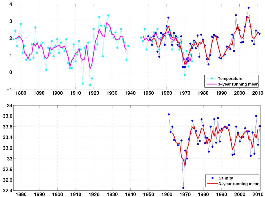
Figure 15. Timeseries of mean temperature (top) and salinity (bottom) on top of Fylla Bank (Station 2, 0–40 m) in the middle of June for the period 1950–2011. The red curve is the 3 year running mean value. Statistics is shown in Table 1. The timeseries for temperature (top, magenta/purple) is extended back to 1876 using Smed-data for area A1 (Smed, 1978). See Ribergaard et al. (2008) for details.
