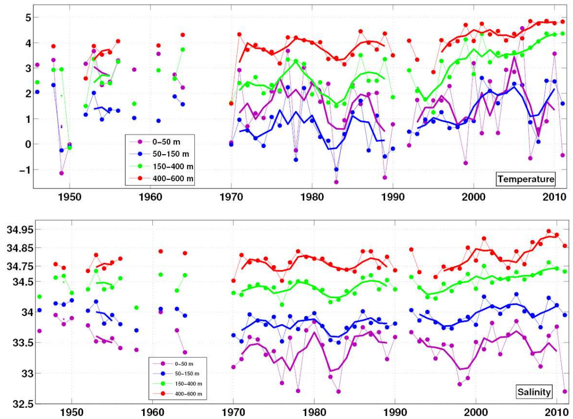
Figure 21. Timeseries of mean temperature (top) and mean salinity (bottom) for the period 1946–2011 in four different depth intervals west of “Store Hellefiskebanke” (Sisimiut, st.5) over the continental slope. The thick curves are the 3 year running mean values. Note the change in scales at 34.75 for salinity. Statistics is shown in Table 4.
