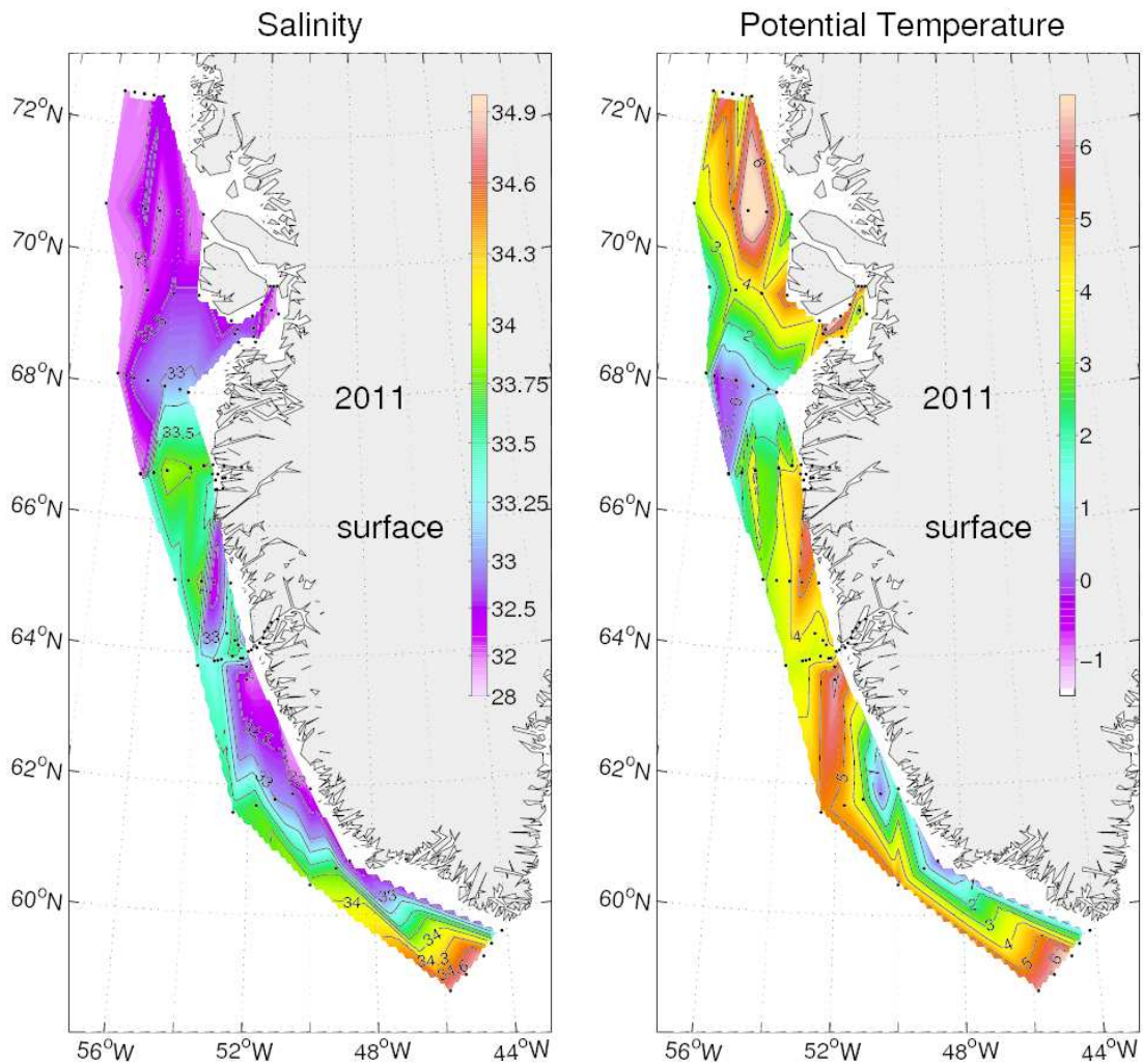
Figure 16. Surface salinity (left) and temperature (right) observed in 2011 taken June 15 – July 13.
