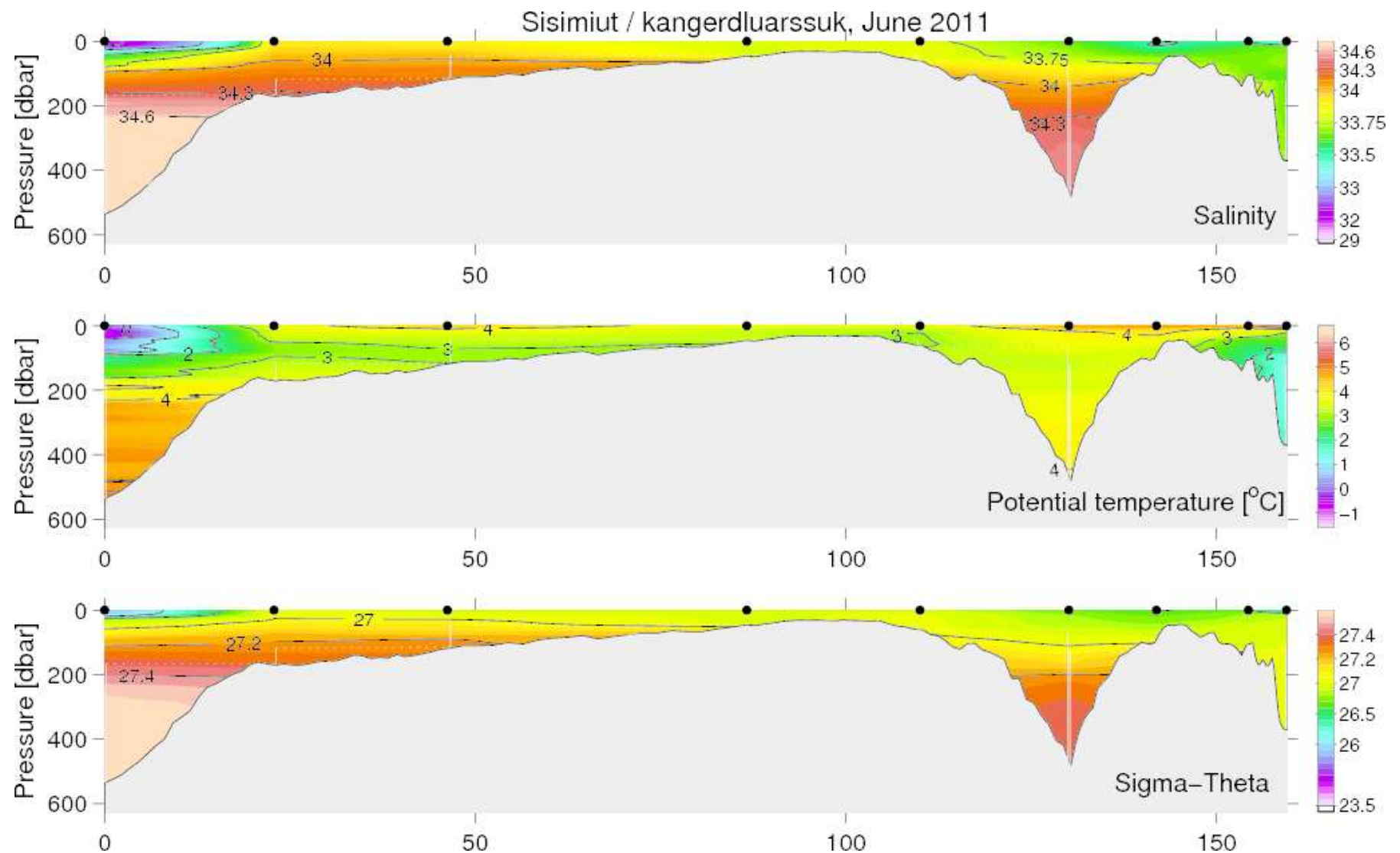
Figure 46. Vertical distribution of temperature, salinity and density at the Kangerdluarssuk fjord, June 28–29, 2011. Sisimiut section left.
