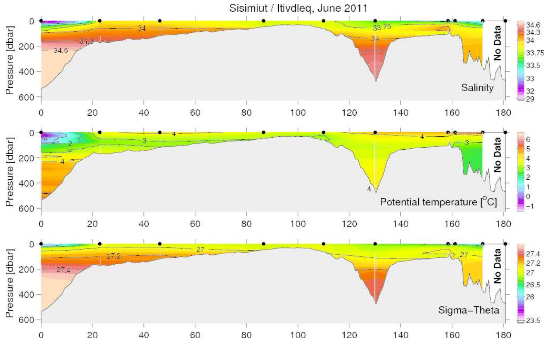
Figure 47. Vertical distribution of temperature, salinity and density at the Itivdleq fjord, June 28–29, 2011. Sisimiut section left.
