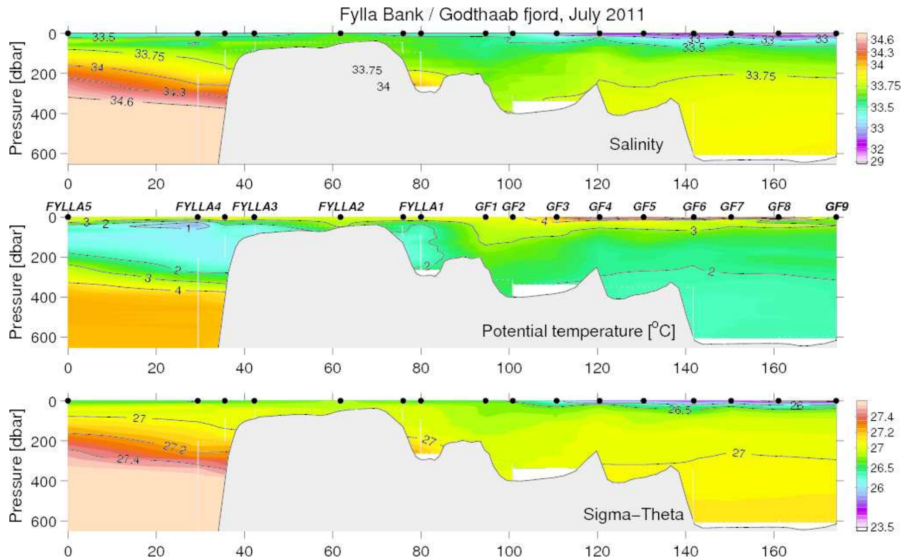
Figure 43. Vertical distribution of temperature, salinity and density at the Godthaab fjord section, July 01, 2011. Fylla Bank section left (as in Figure 31).
