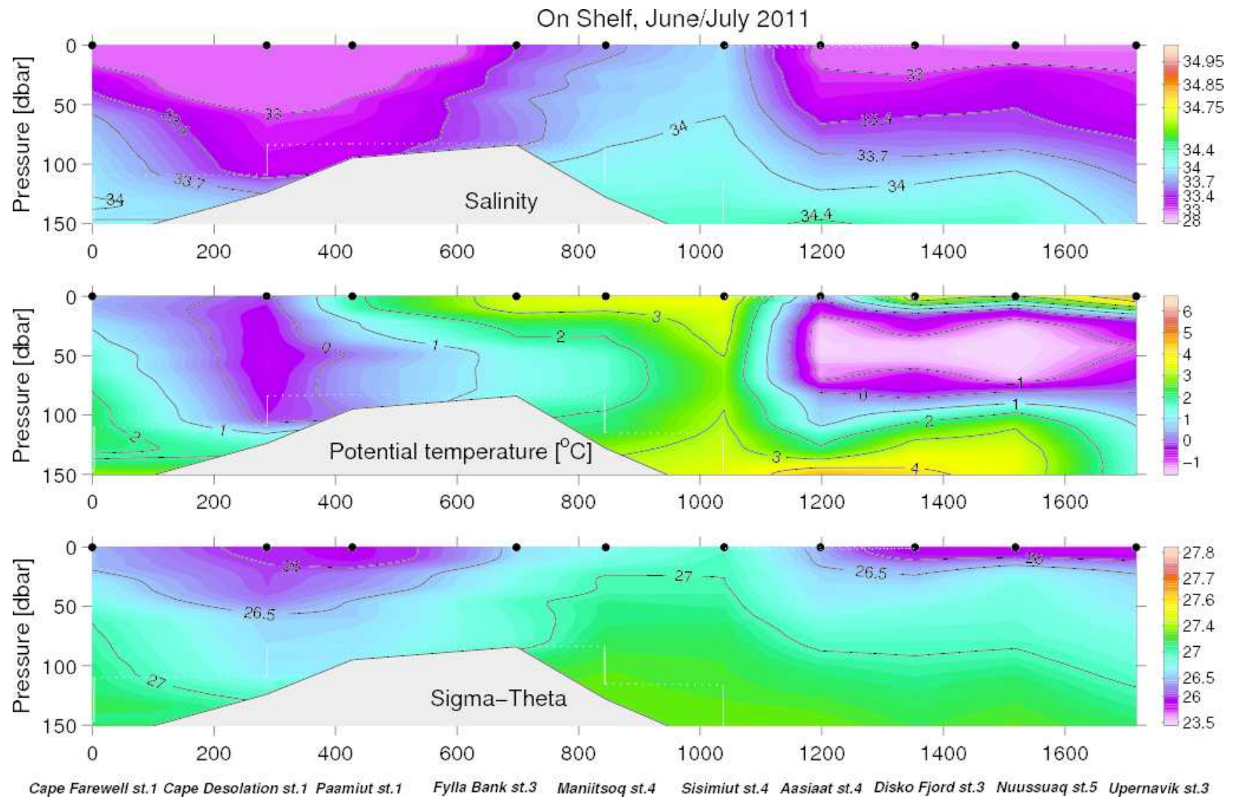
Figure 27. Vertical distribution of temperature, salinity and density over the shelf banks from Cape Farewell to Sisimiut, Cape Farewell to Upernavik, June 18–July 12, 2011.
