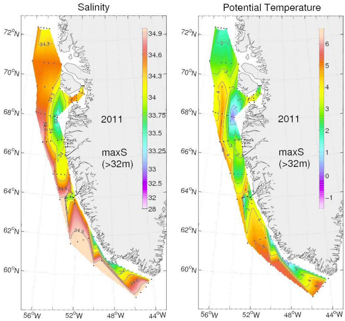
Figure 25. Salinity (left) and temperature (right) observed in 2011 (June 15 – July 13) at the depth of maximum salinity disregarding the upper 32 meters.
