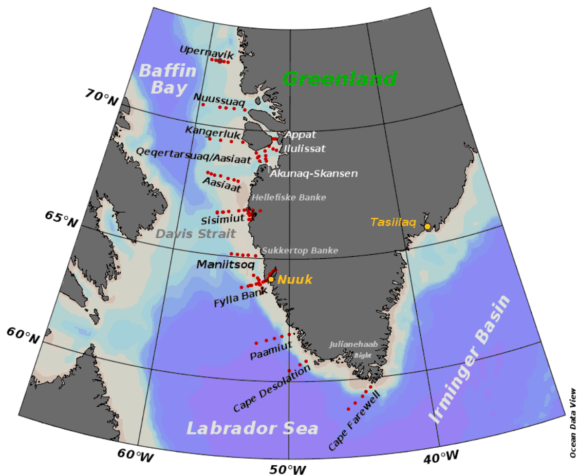
Figure 1. Position of the oceanographic sections off West Greenland where measurements were performed in 2011. Map produced using Ocean Data View (Schlitzer, 2007).
