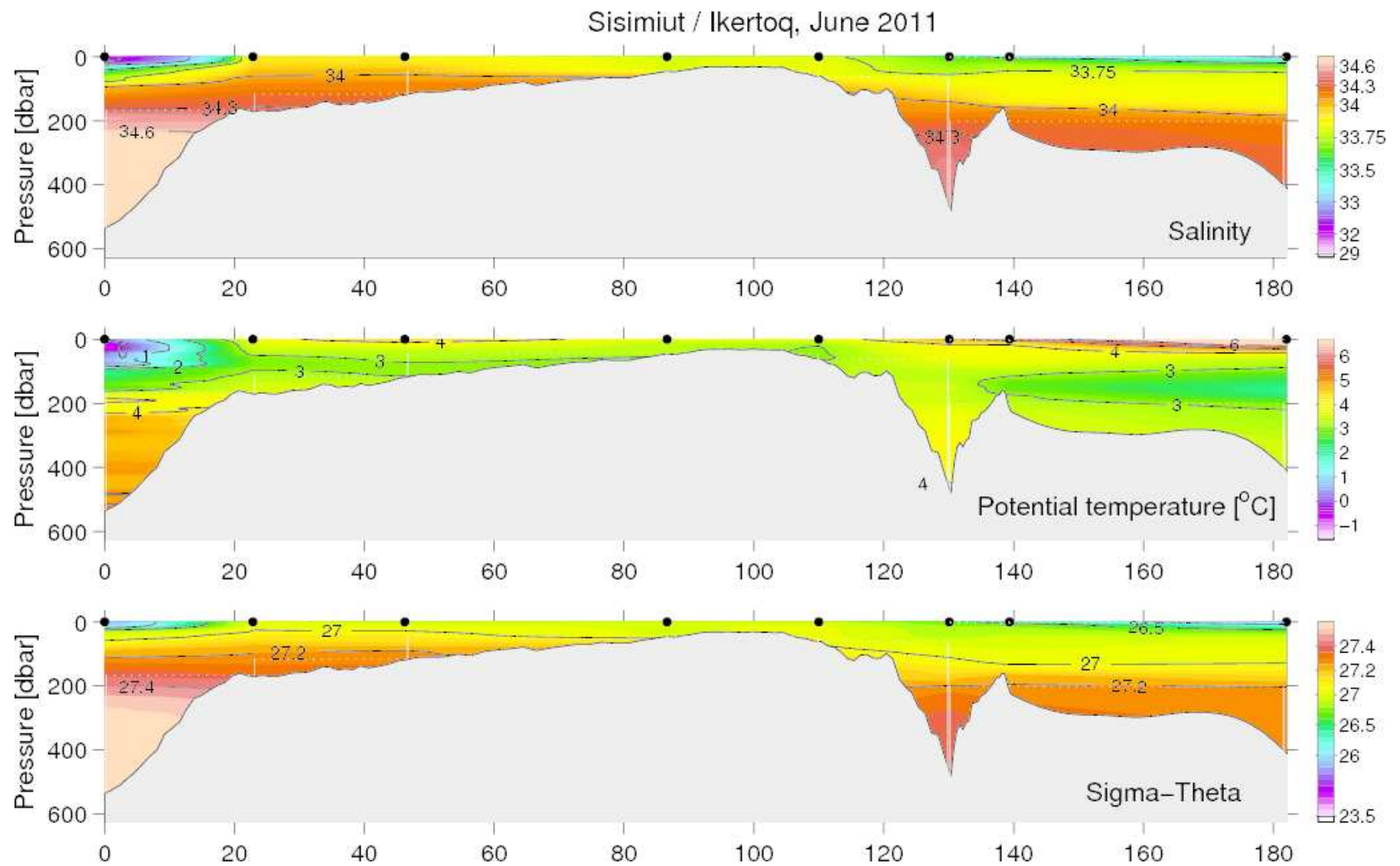
Figure 45. Vertical distribution of temperature, salinity and density at the Ikertoq fjord, June 28–29, 2011. Sisimiut section left
