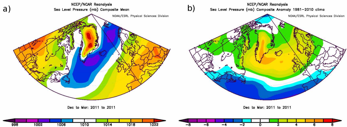
Figure 8. a) Winter (DJFM) sea level pressure for 2010/11 in the North Atlantic region. b) Sea level pressure anomaly. NCEP/NCAR re-analysis (from http://www.esrl.noaa.gov/psd/ ).
