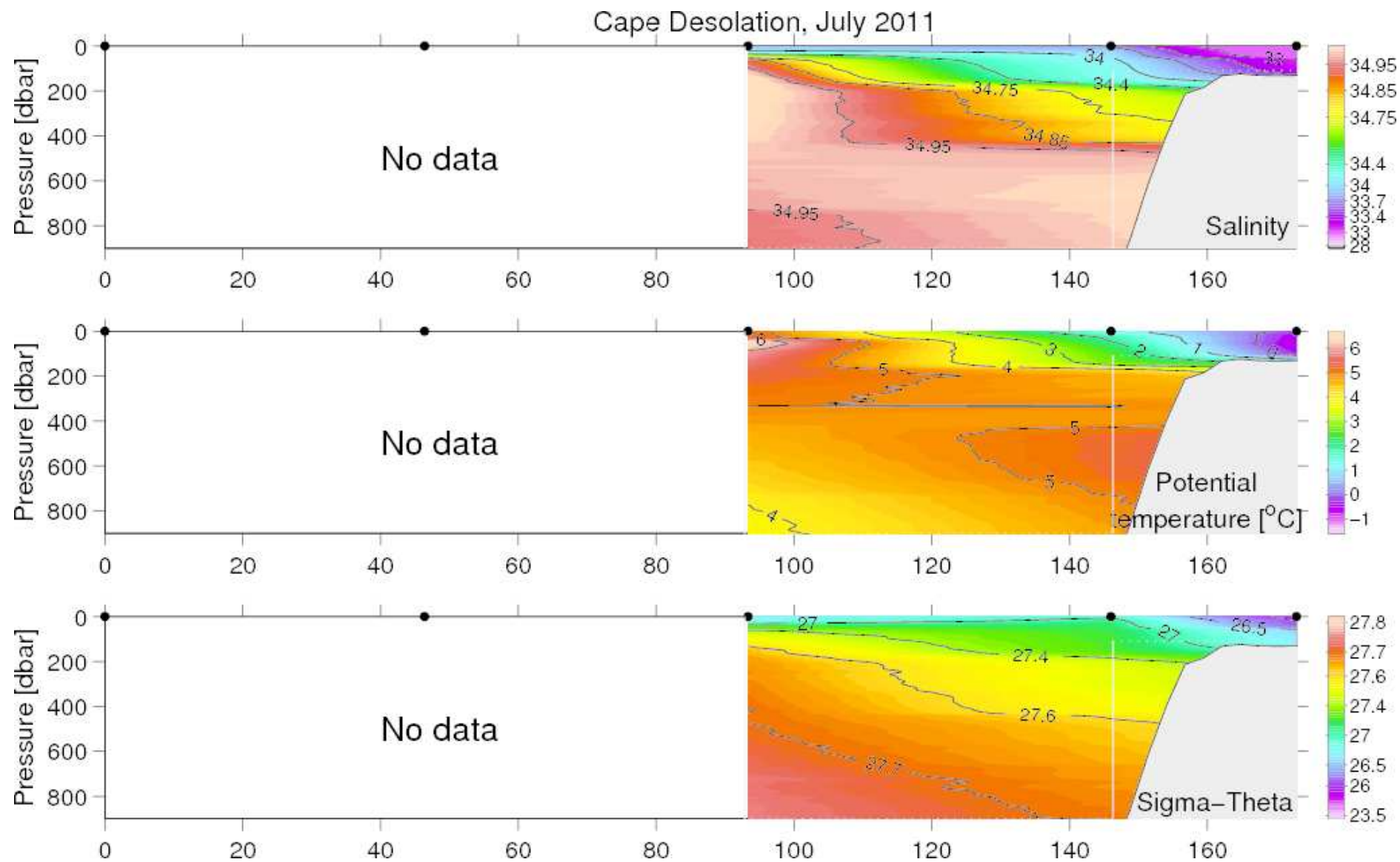
Figure 29. Vertical distribution of temperature, salinity and density at the Cape Desolation section, July 08–09, 2011.
