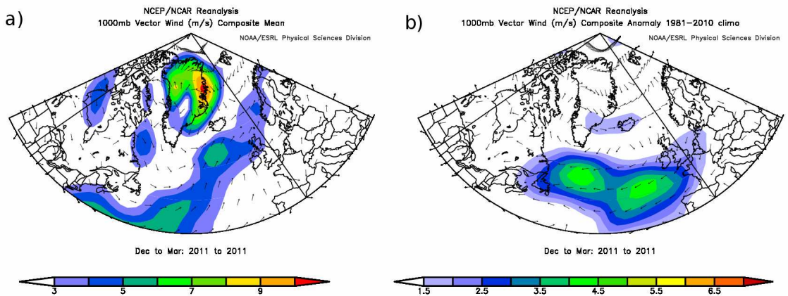
Figure 9. a) Winter (DJFM) wind (left) for 2010/11 in the North Atlantic region. b) Wind anomaly. NCEP/NCAR re-analysis (from http://www.esrl.noaa.gov/psd/ ).
