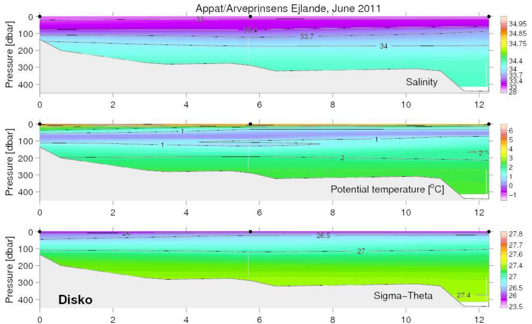
Figure 42. Vertical distribution of temperature, salinity and density at the Appat (Arveprinsens Ejlande) section, June 28–29, 2011.
