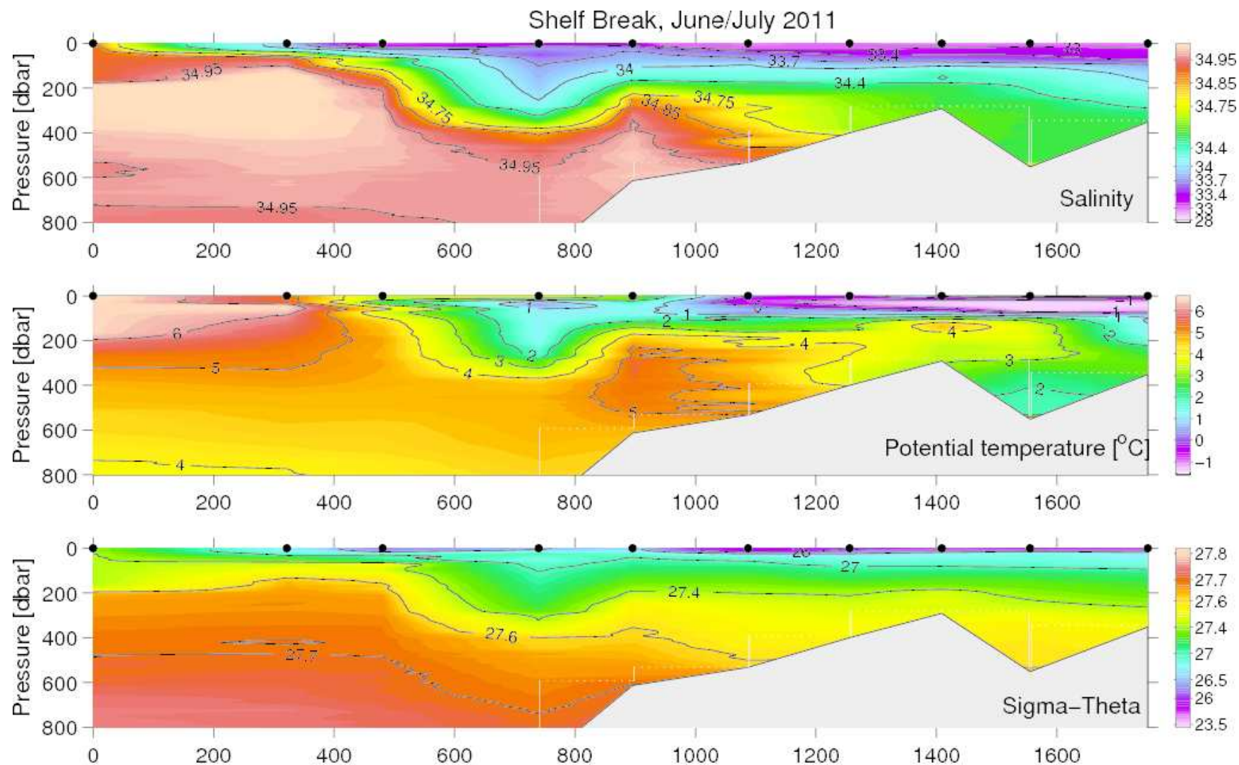
Figure 26. Vertical distribution of temperature, salinity and density over the continental shelf break from Cape Farewell to Upernavik, June 18–July 12, 2011.
